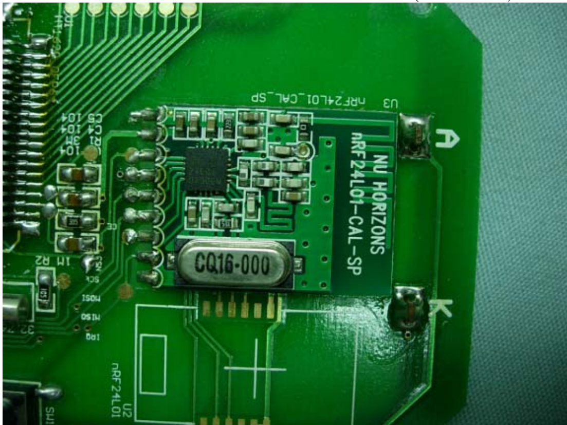
Figure 5 Internal View (RF Modular, Front View)
