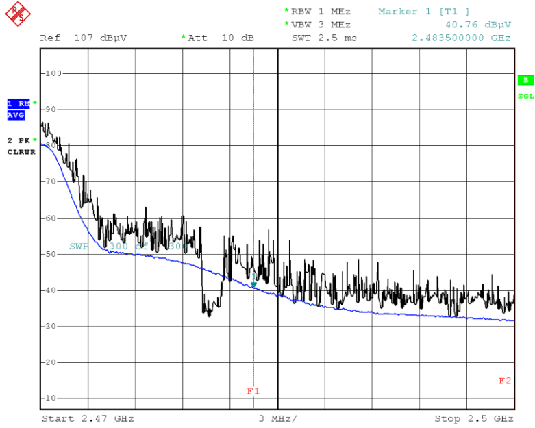
Radiated Restricted Band Edges plot – Average Reading (802.11n Ch.11)
