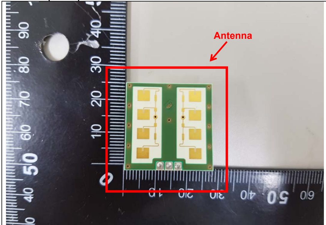
Antenna (Radar)
