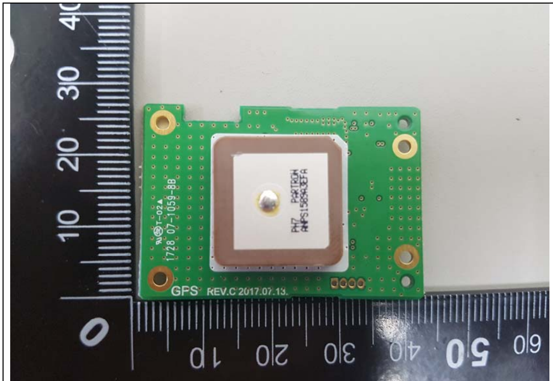
GPS Board Rear
