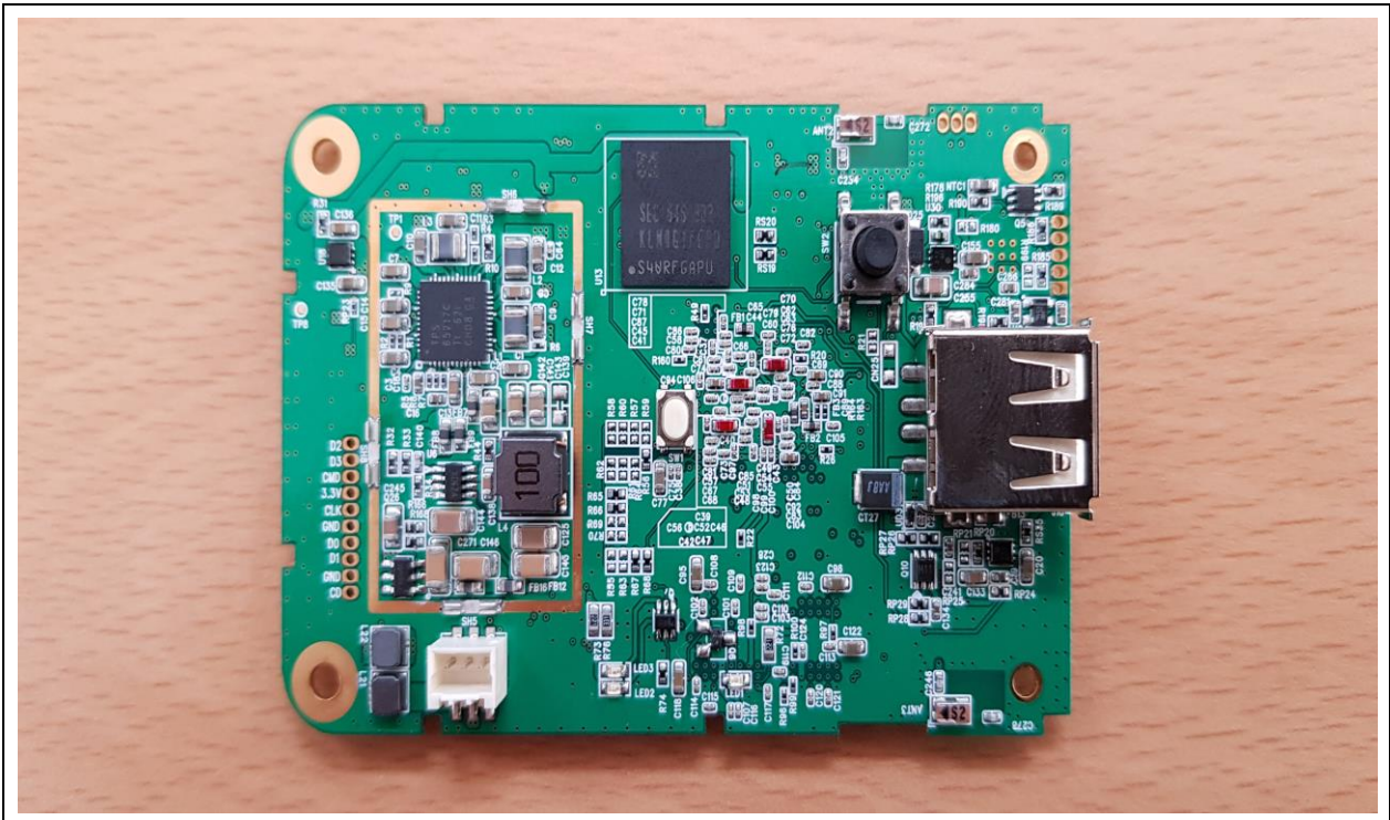
PCB Rear
