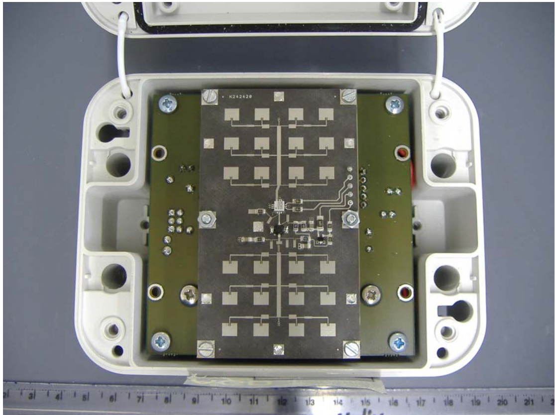
Assembled PCBs Mounted In case
