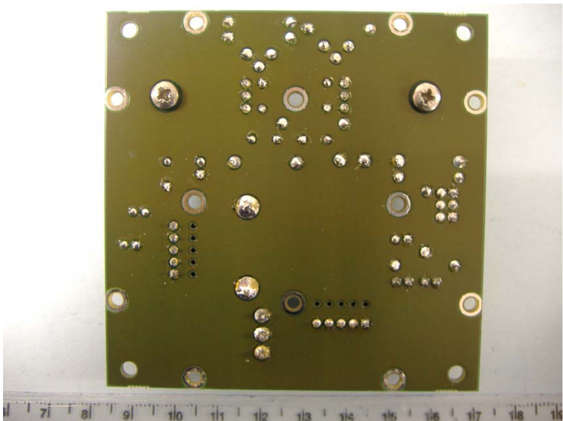
Control PCB Track Side
