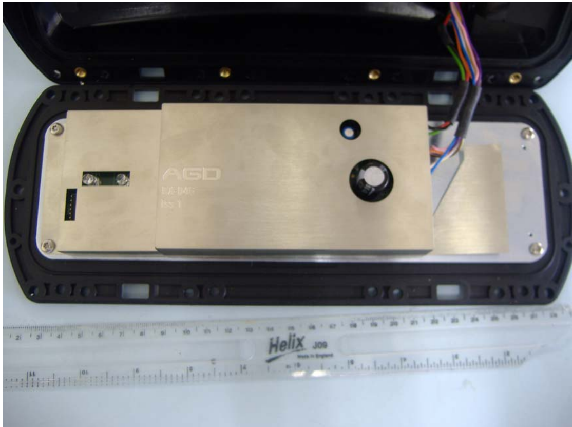
Case Open Can Mounted
