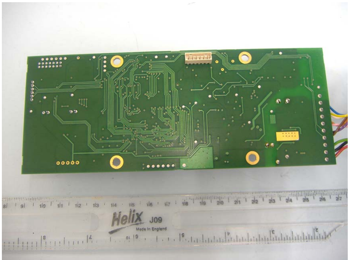
Power Supply and Data Capture PCB Track Side
