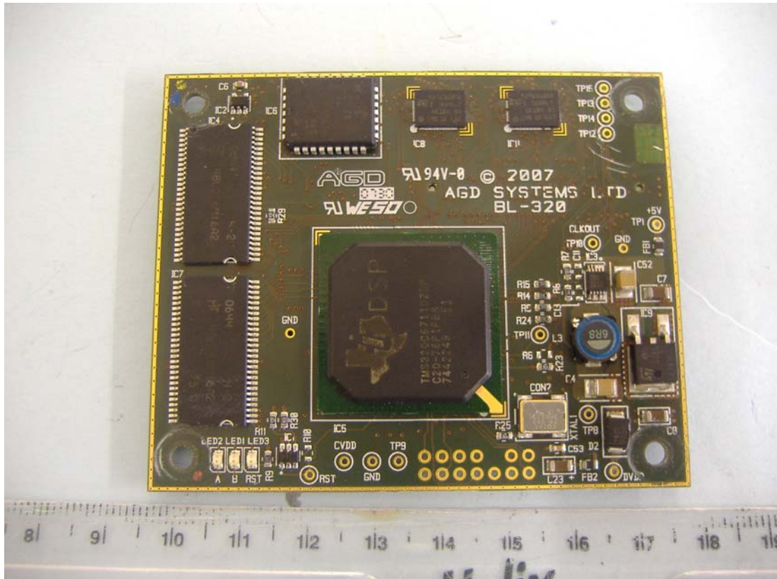
DSP PCB Component Side
