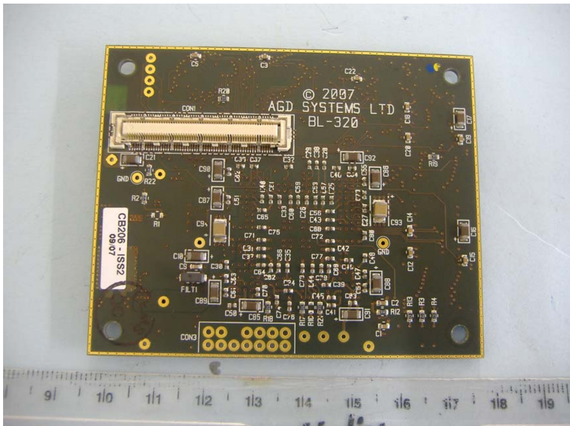
DSP PCB Track Side
