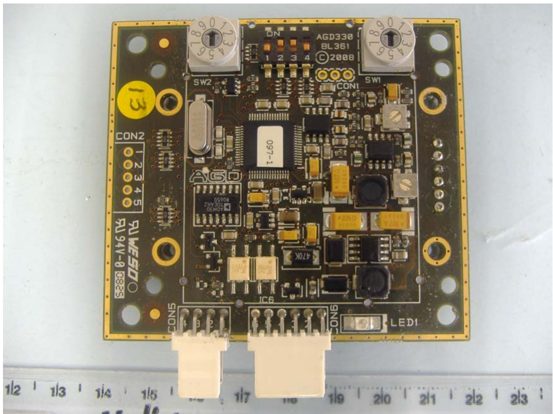
Component Side Of PCB Can Removed
