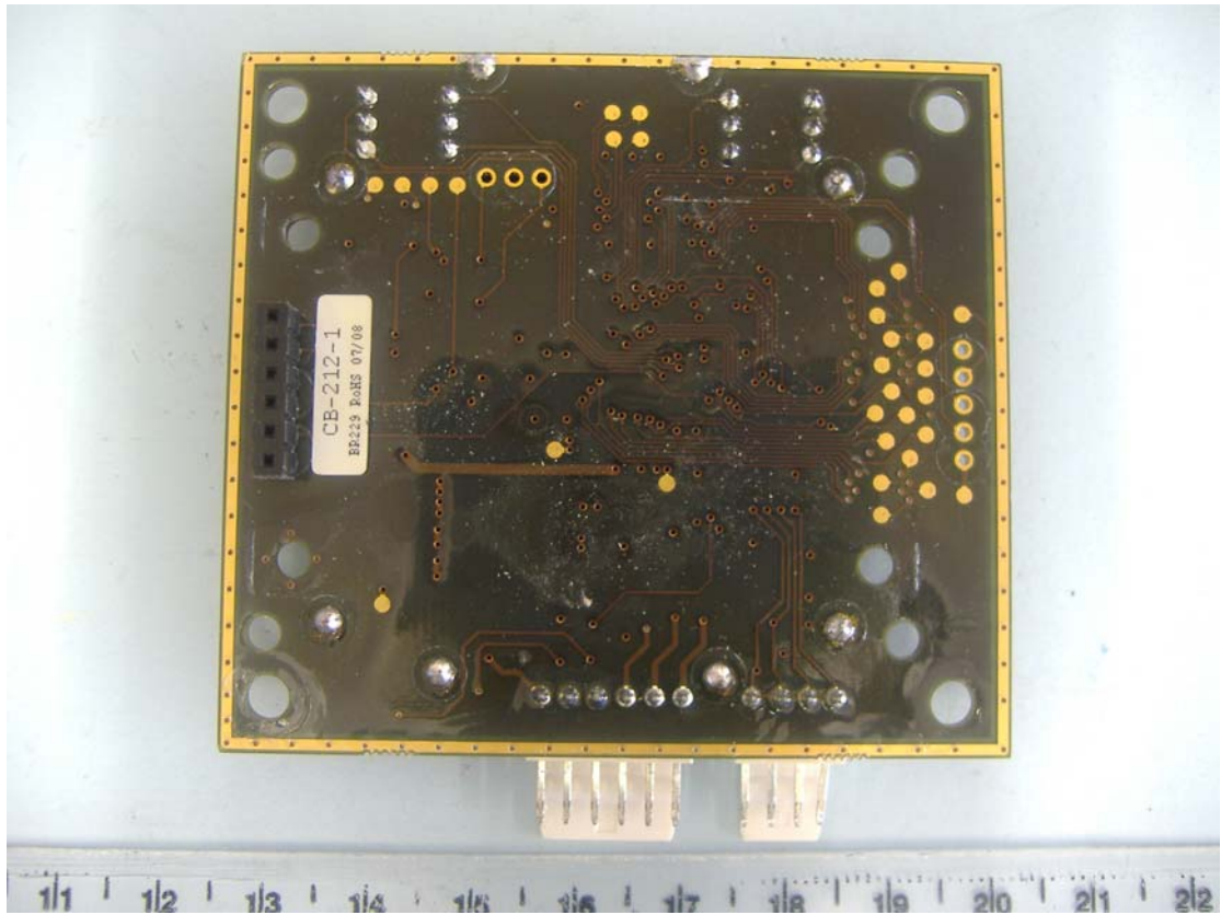
Track Side Of PCB RF Module Removed
