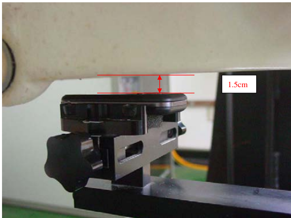
Picture B14: Body-worn Position-slide down (towards phantom, the distance from handset to the bottom of the Phantom is 1.5cm)
