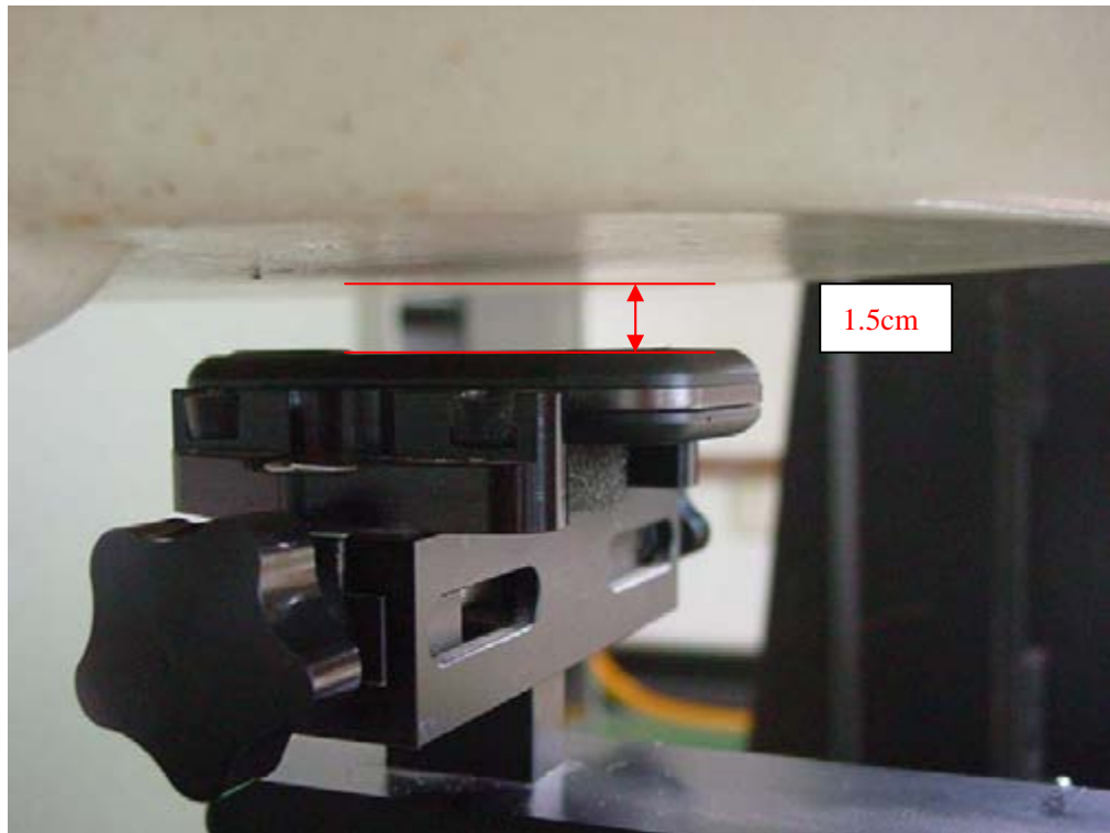
Picture B13: Body-worn Position-slide down (towards ground, the distance from handset to the bottom of the Phantom is 1.5cm)
