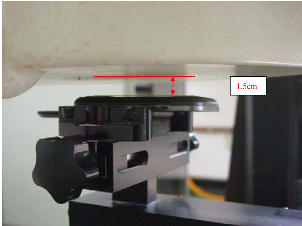
Picture B11: Body-worn Position-slide up (towards ground, the distance from handset to the bottom of the Phantom is 1.5cm)
