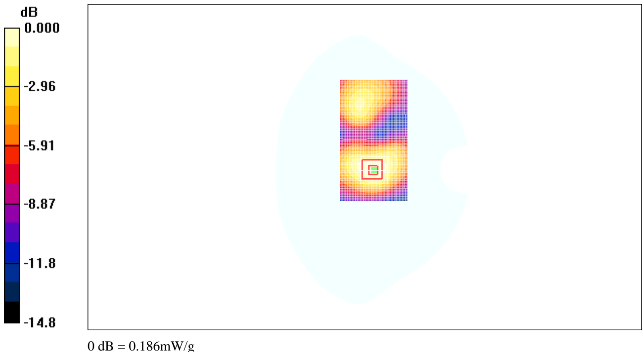
Fig. 73 1900 MHz CH512
