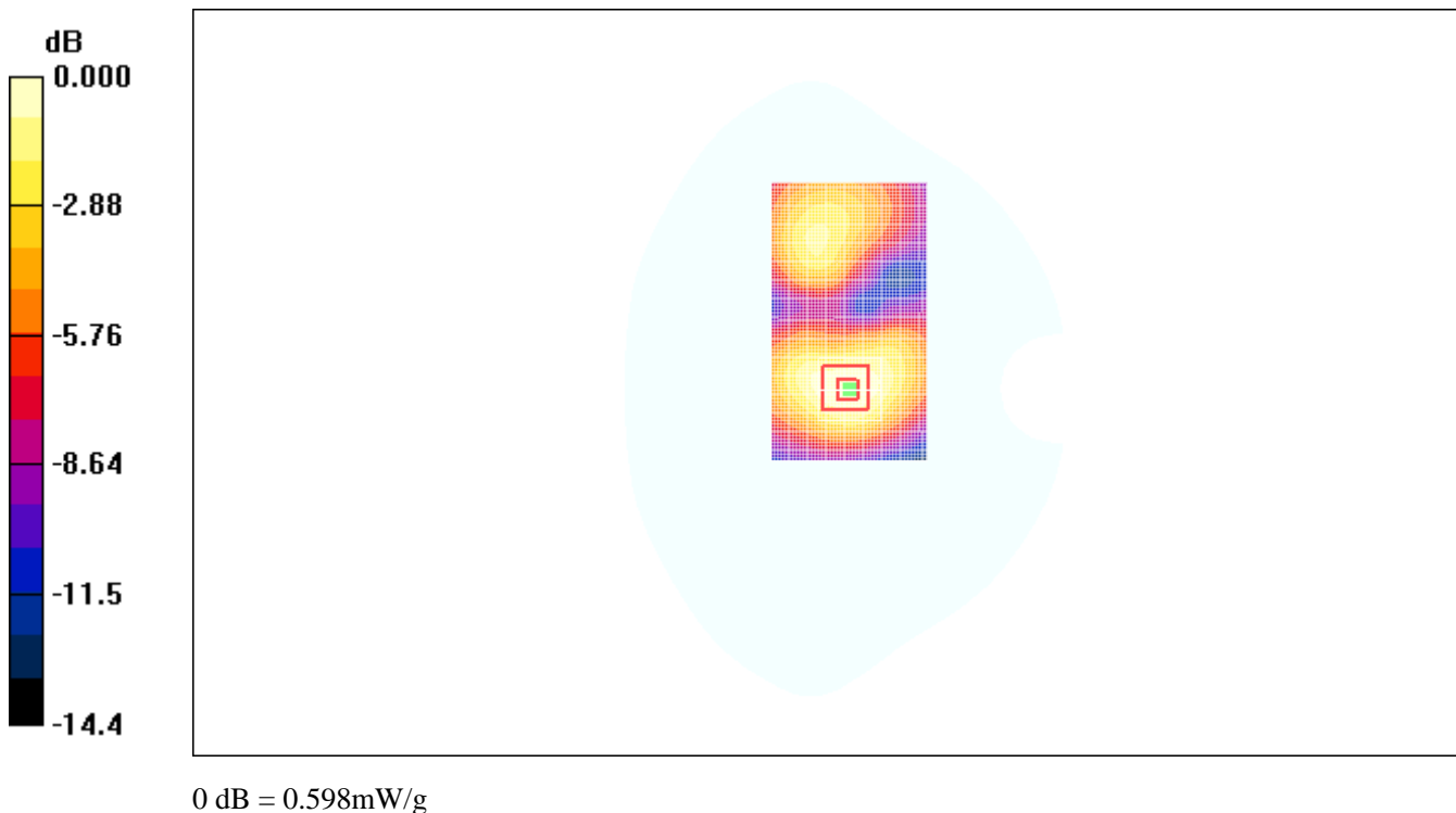
Fig. 59 1900 MHz CH512
