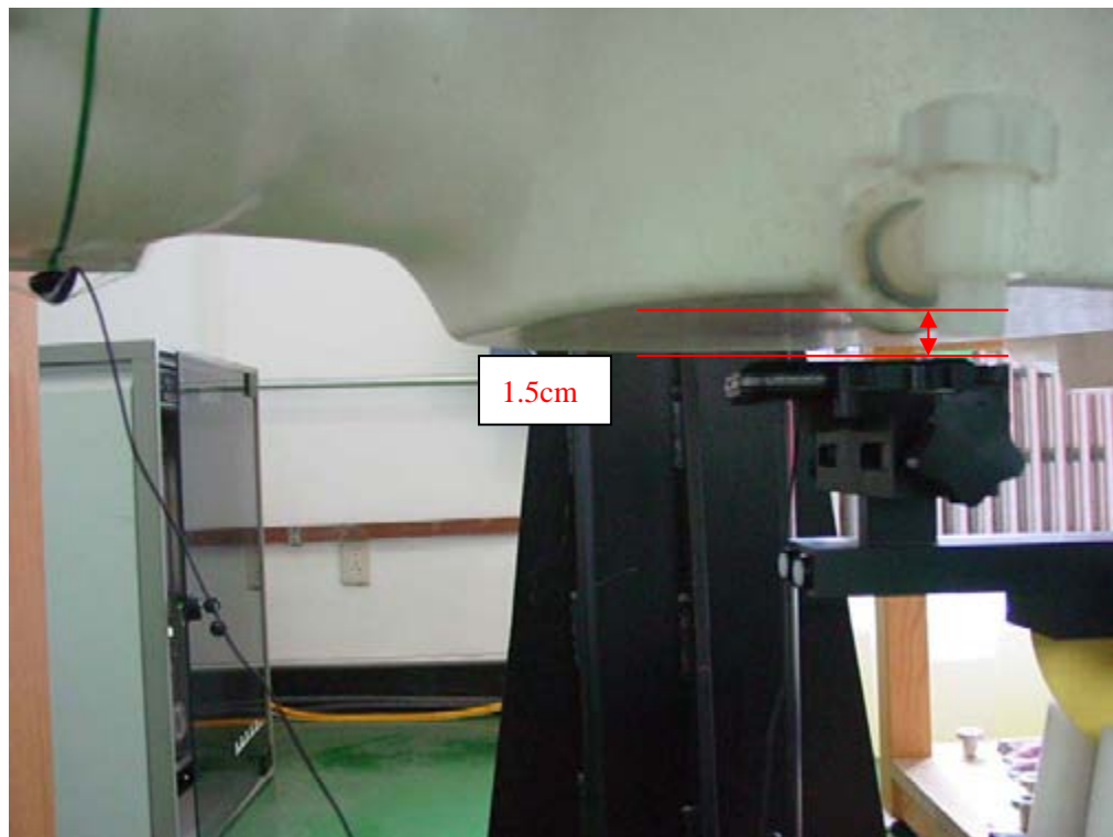
Picture B16: Body-worn Position with Headset-slide down (towards ground, the distance from handset to the bottom of the Phantom is 1.5cm)
