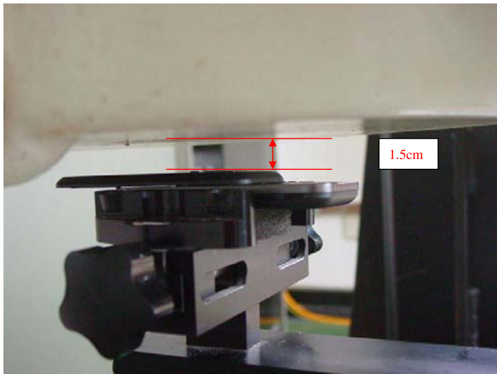
Picture B12: Body-worn Position-slide up (towards phantom, the distance from handset to the bottom of the Phantom is 1.5cm)
