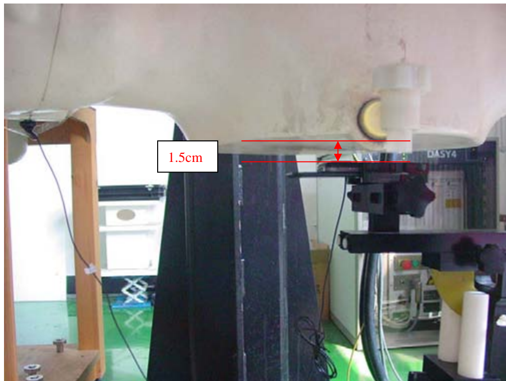
Picture B15: Body-worn Position with Headset-slide up (towards ground, the distance from handset to the bottom of the Phantom is 1.5cm)
