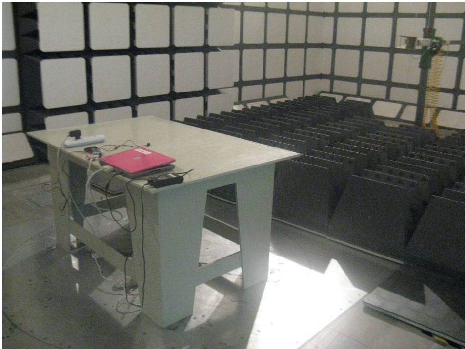
Above 1 GHz: Radiated Emissions - Rear View (Transmitting)
