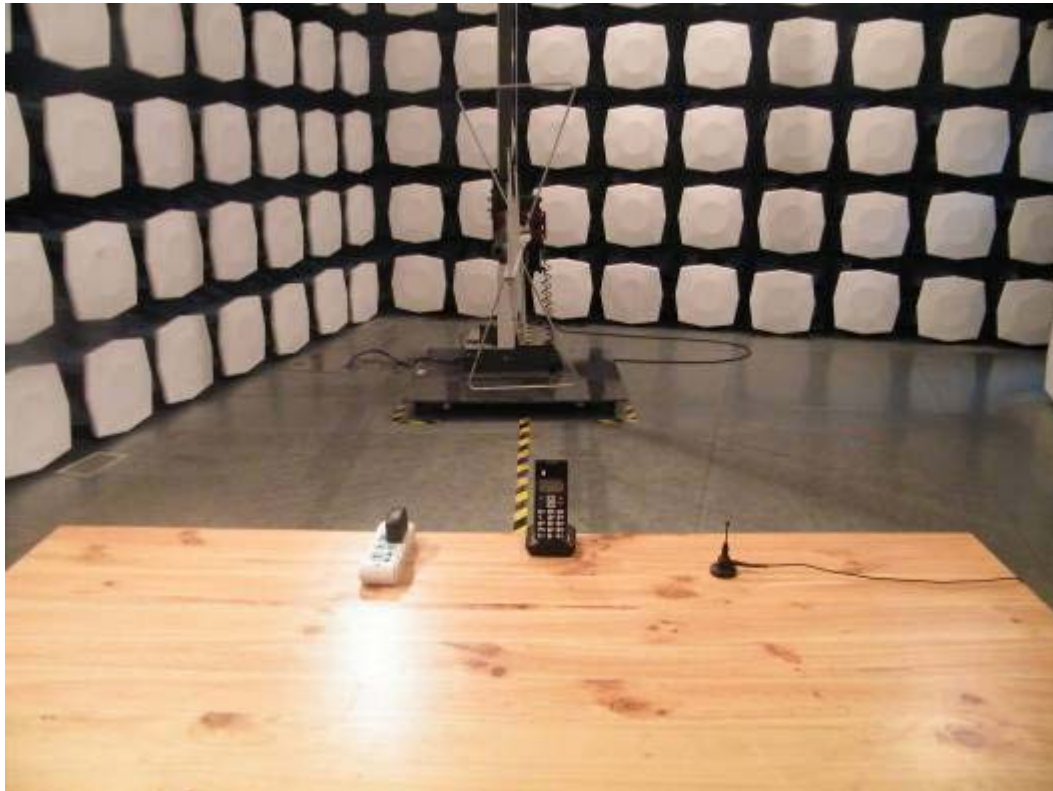
Picture 1-1 EUT with charger base
