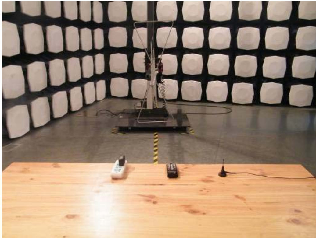
Picture 2-1 EUT with charger base
