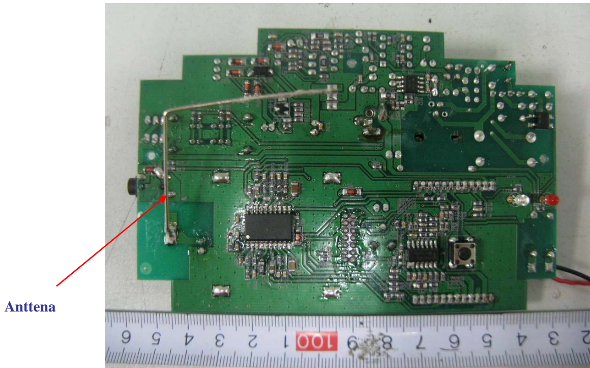
EUT – Base Board Bottom Components View
