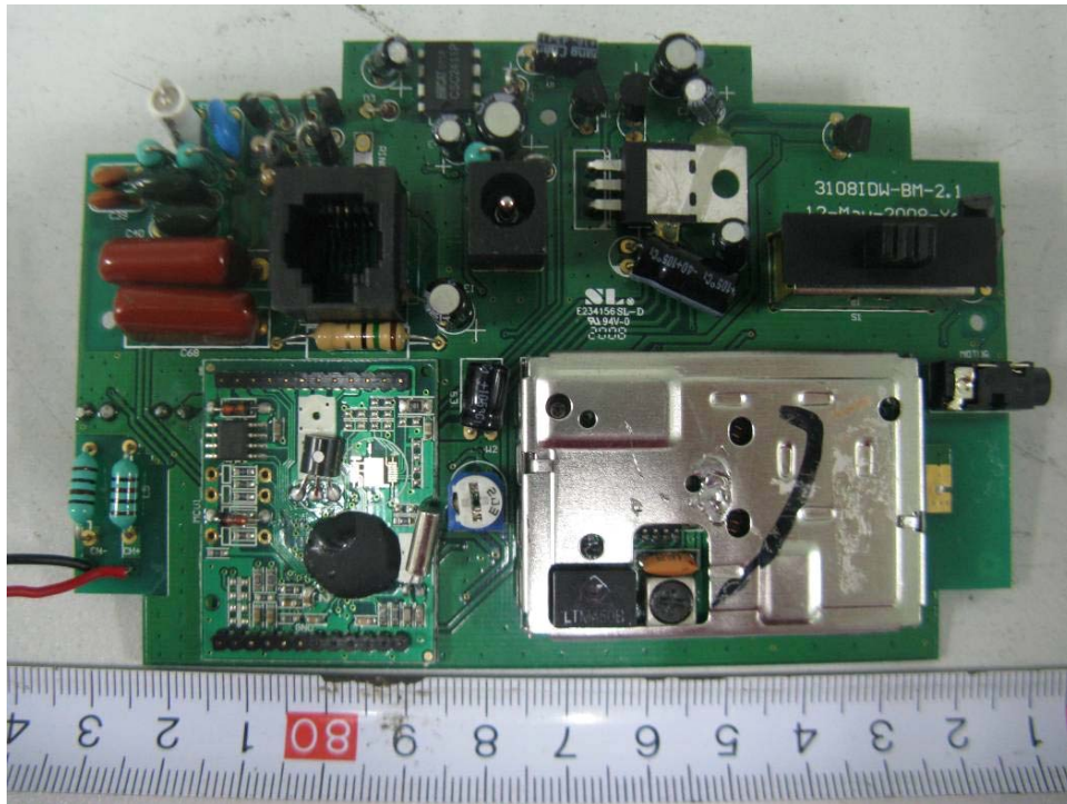
EUT – Base Board Top Components View
