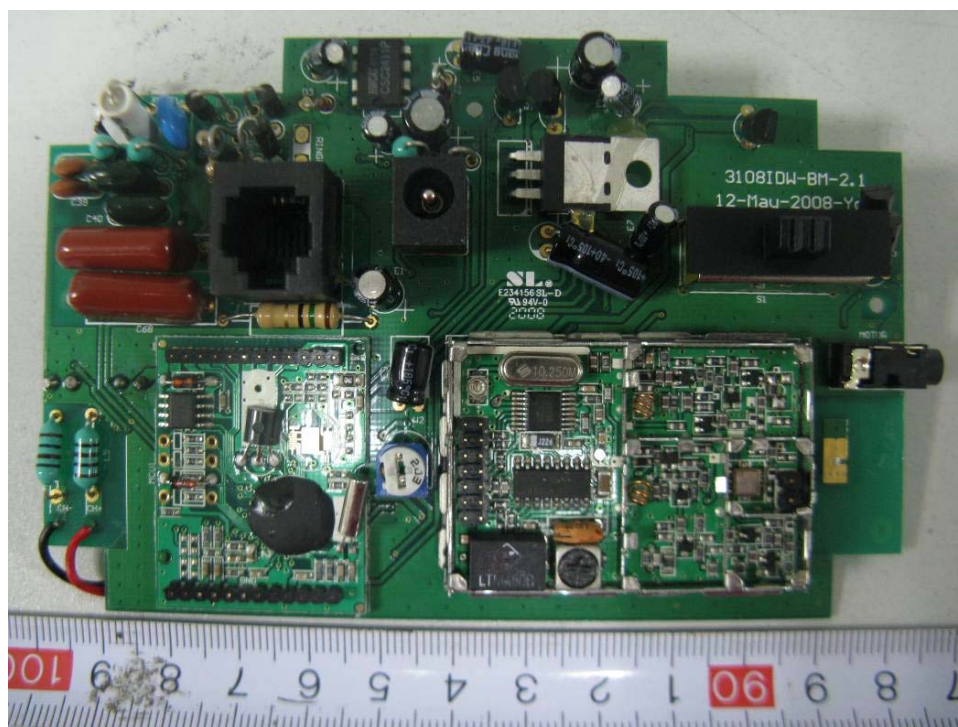
EUT – Base Board Uncover RF View
