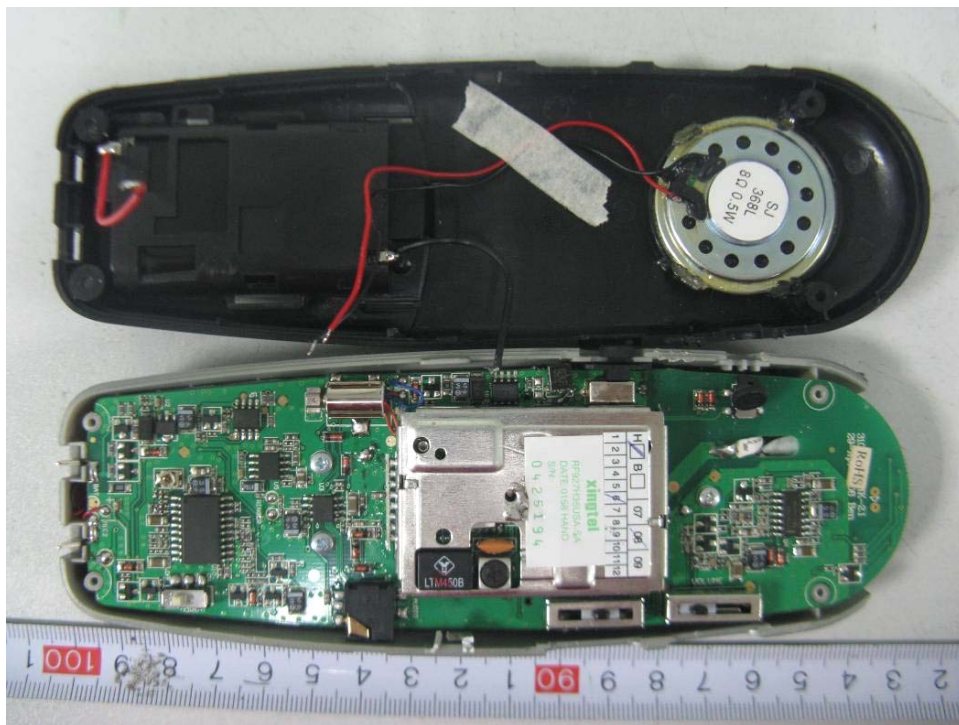
EUT – Handset Cover off View
