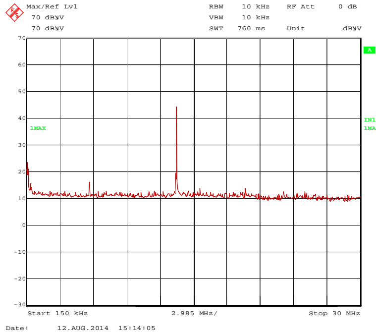
144371_b.wmf: Spurious emissions from 150 kHz to 30 MHz
