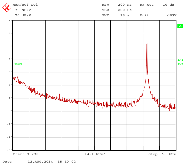
144371_a.wmf: Spurious emissions from 9 kHz to 150 kHz
