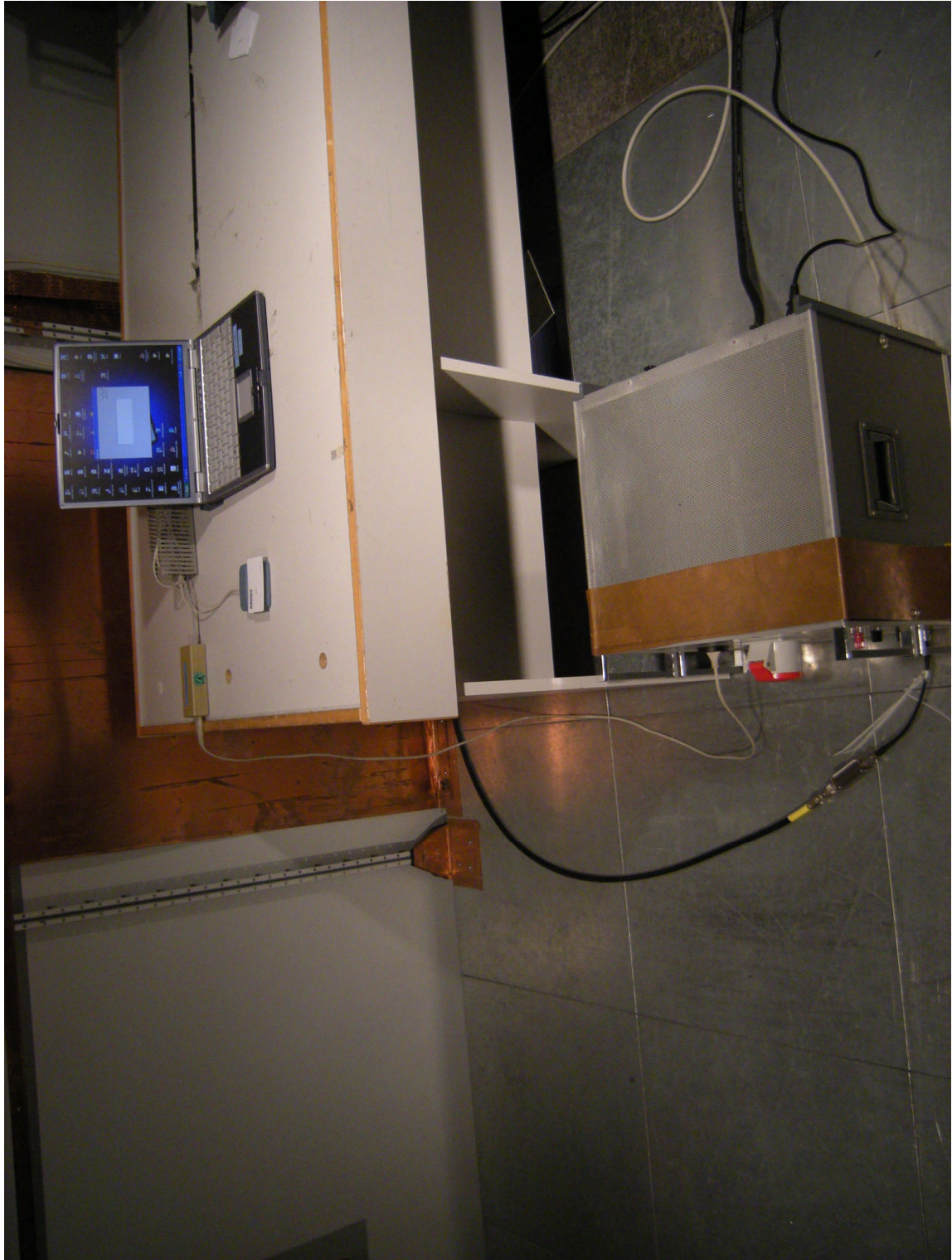
91052emi_c1.jpg Test set-up conducted emissions
