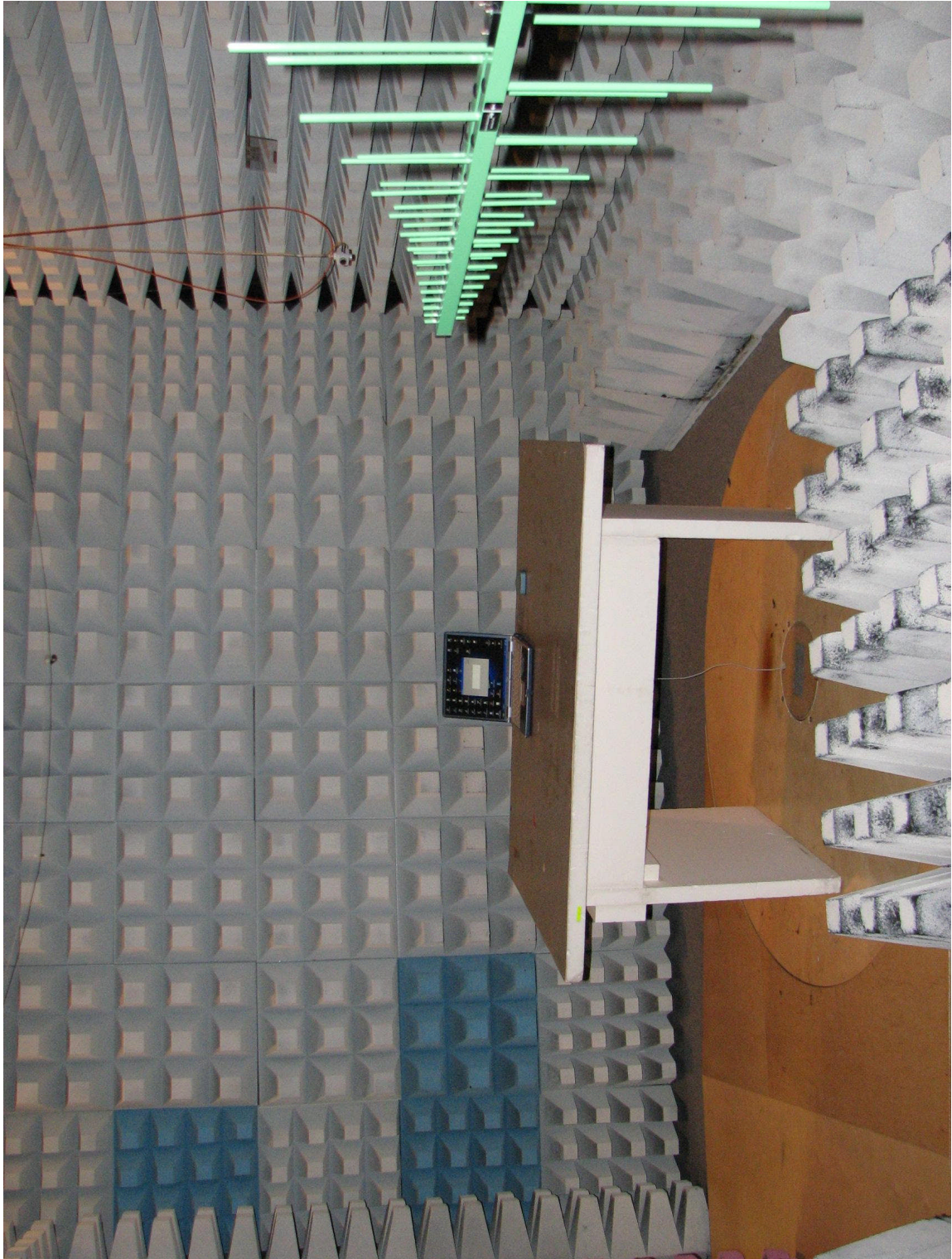
91052emi_fcc9.jpg Test set-up preliminary radiated emissions (E-Field)
