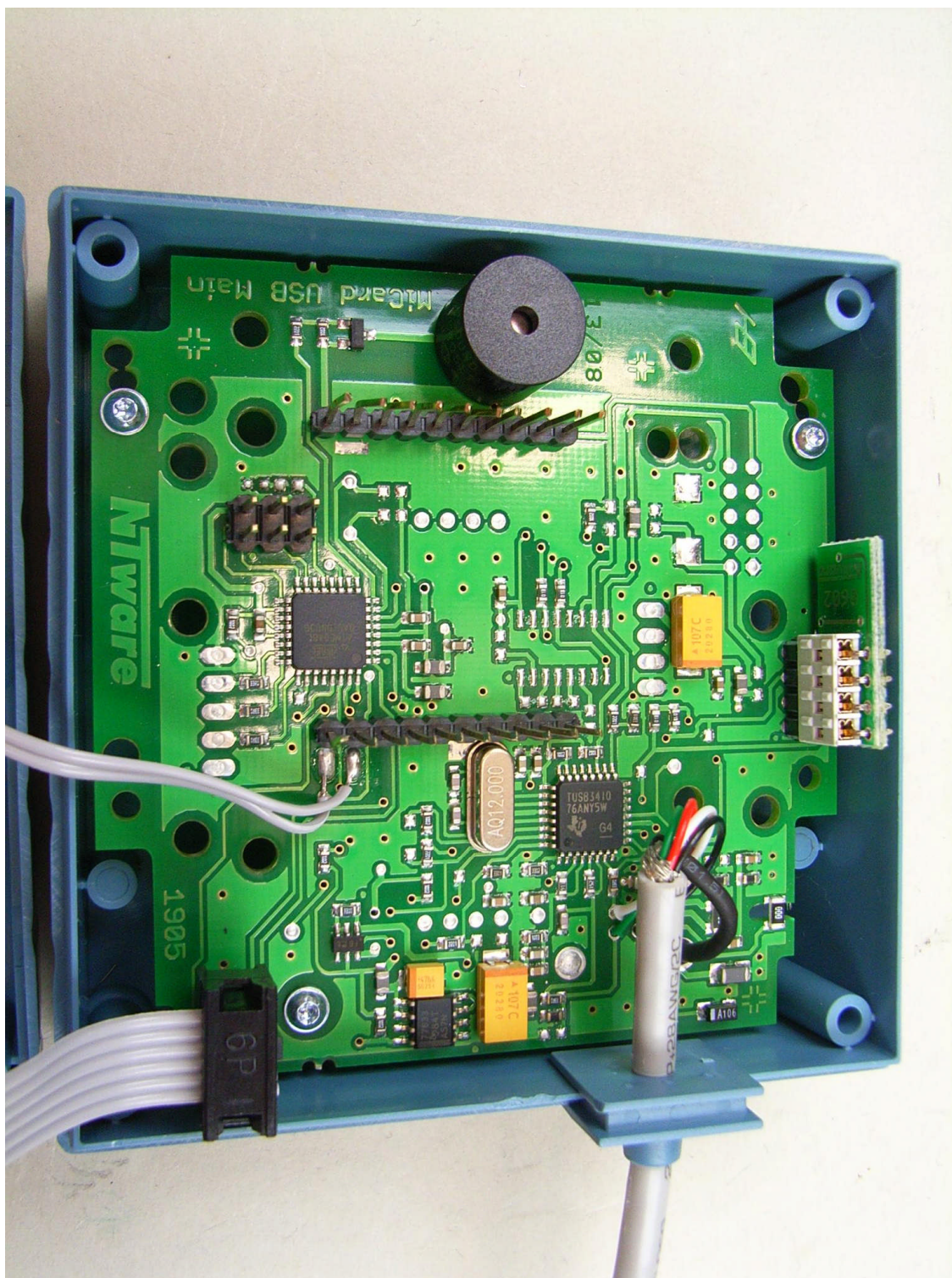
81609eut15: EUT, main-PCB, RF-part removed
