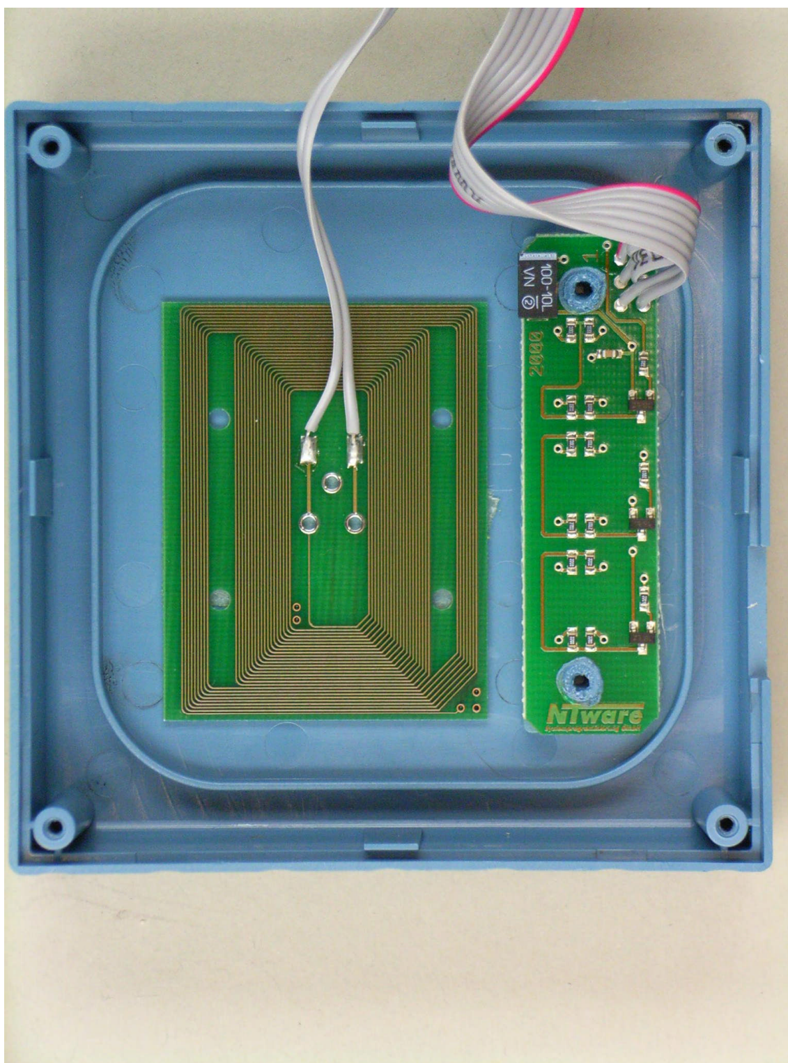
81609eut6: EUT, antenna view
