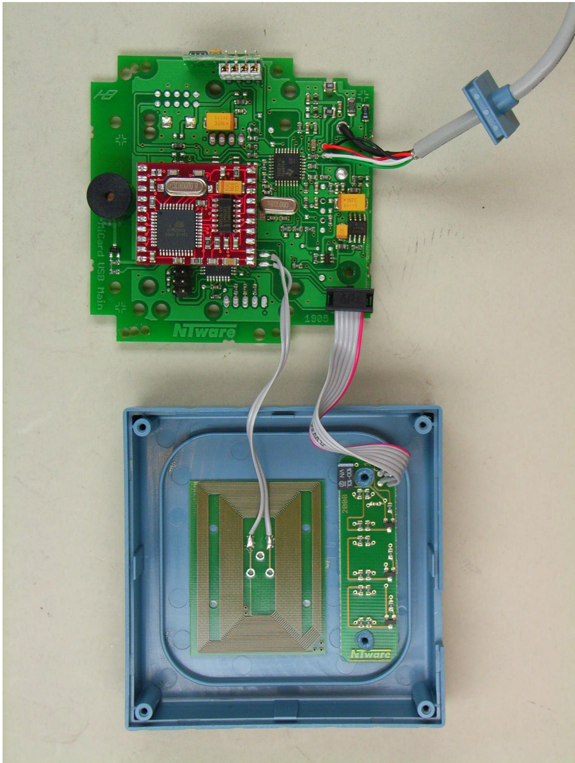
81609eut12: EUT, inside view
