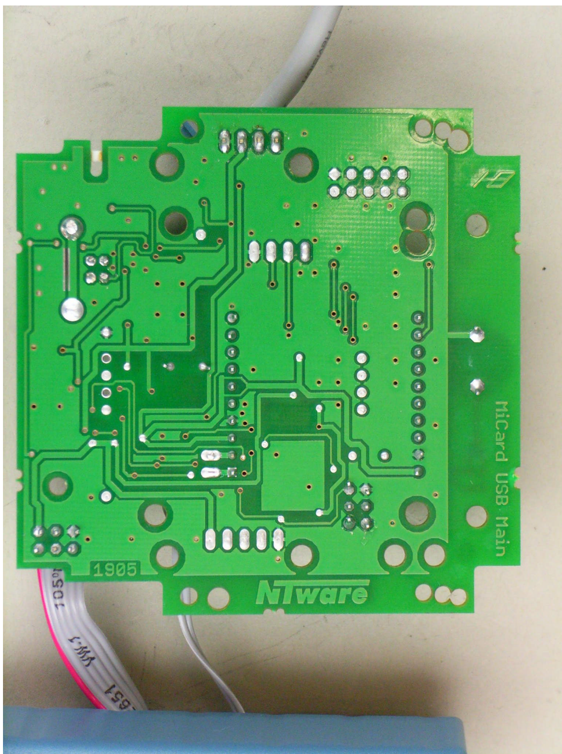
81609eut8: EUT, main-PCB, rear view
