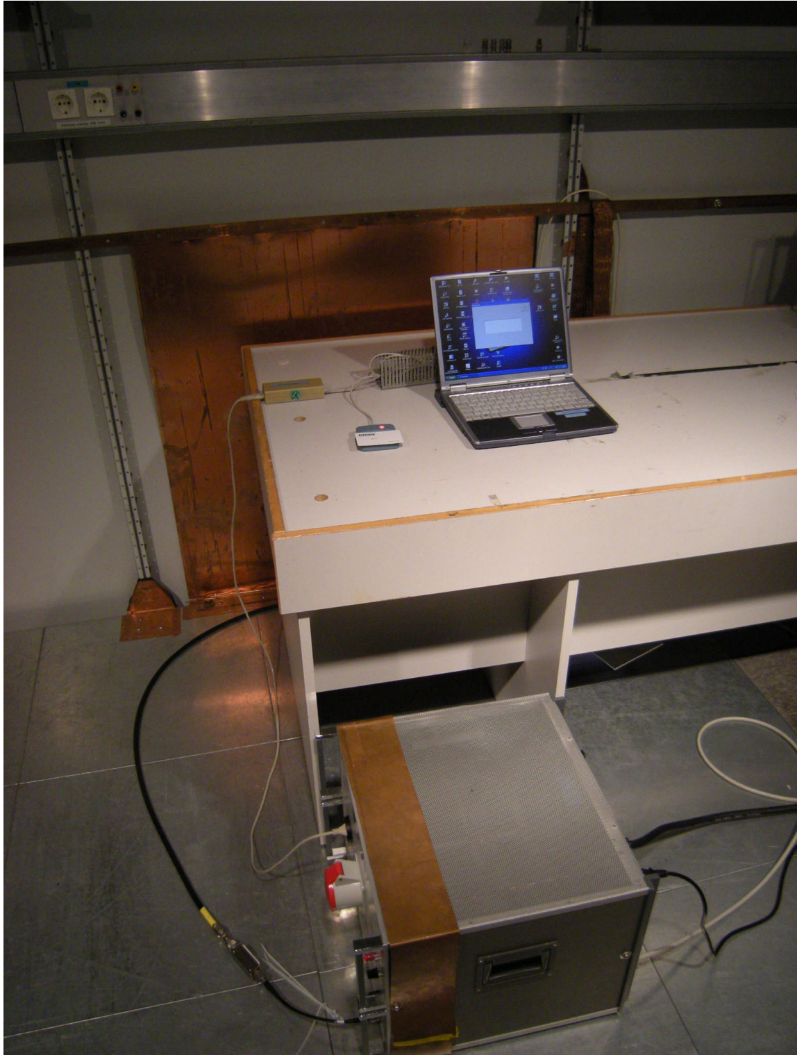
91050emi_c1.jpg Test set-up conducted emissions
