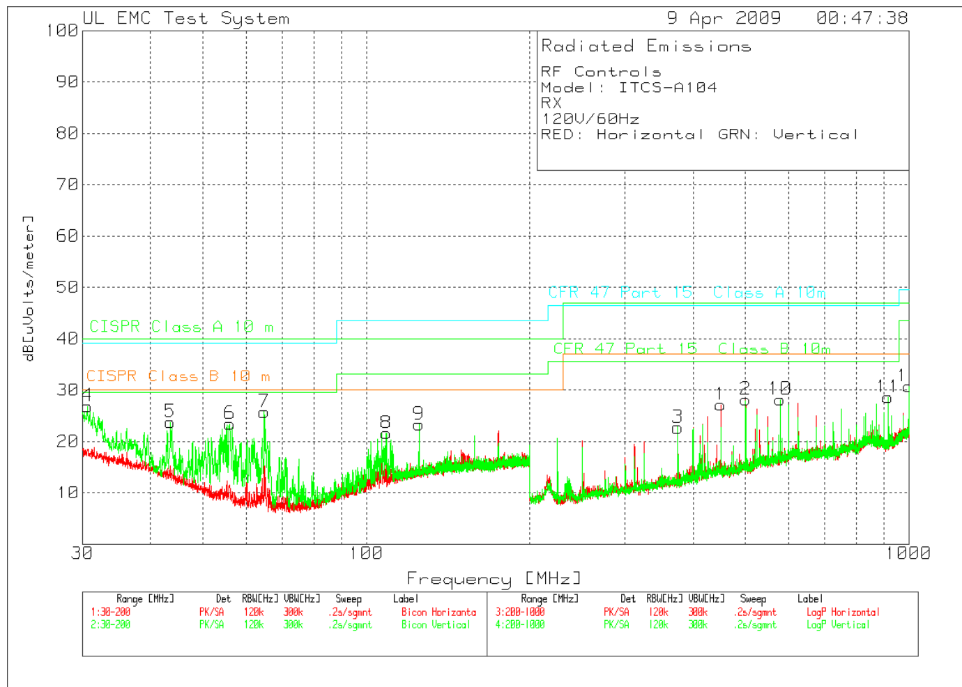
Figure 23 Radiated Emissions Graph 30MHz – 1GHz
