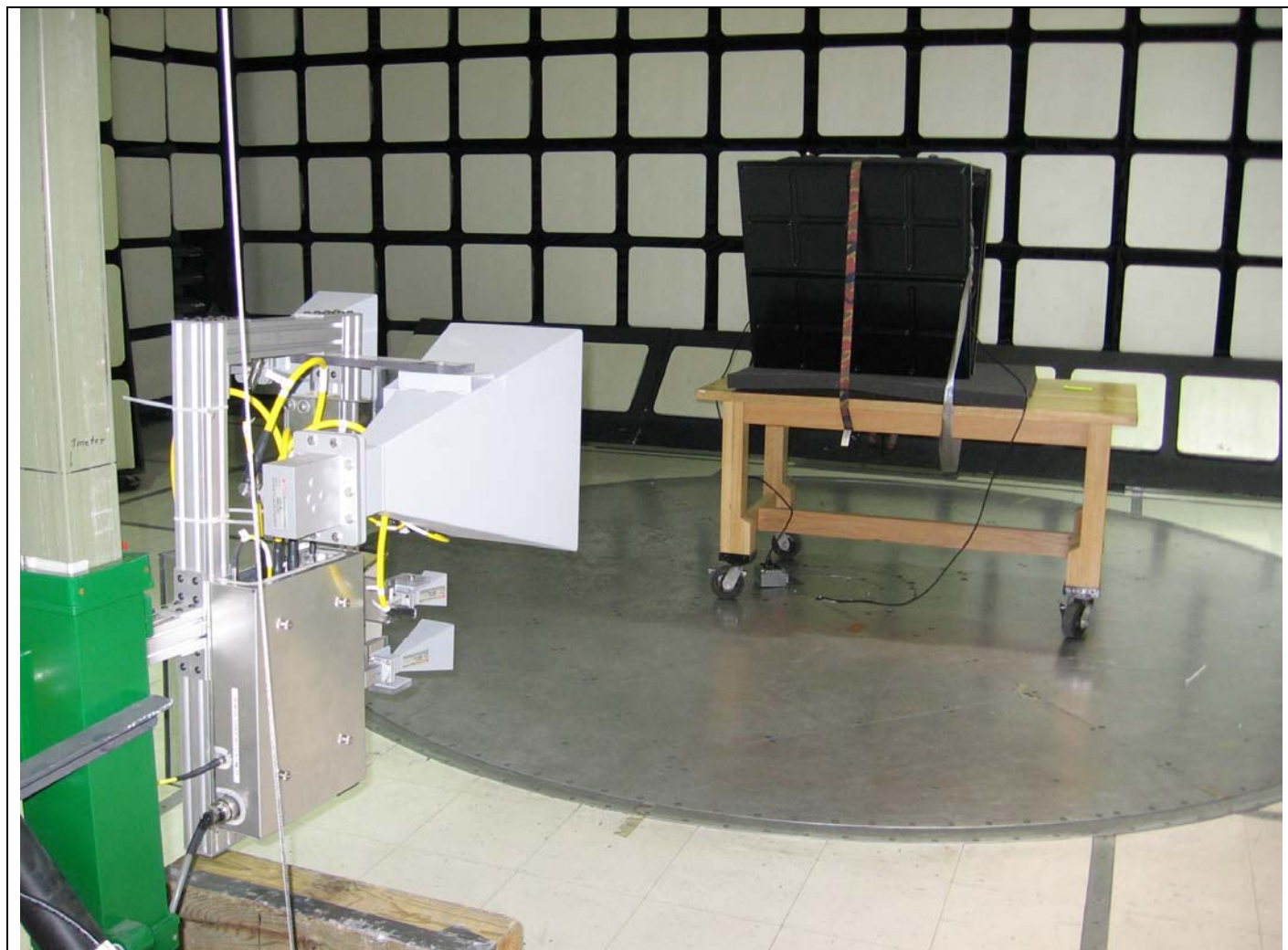
Figure 17 Test setup for SPURIOUS EMISSIONS – Radiated
