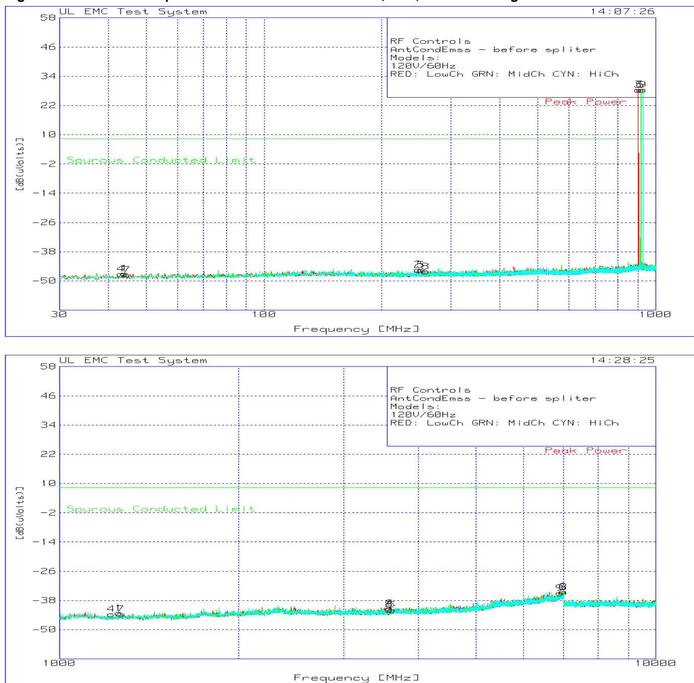
Figure 18 Antenna Port Spurious Emissions Plots TX Mode, Low, Middle and High Channels
