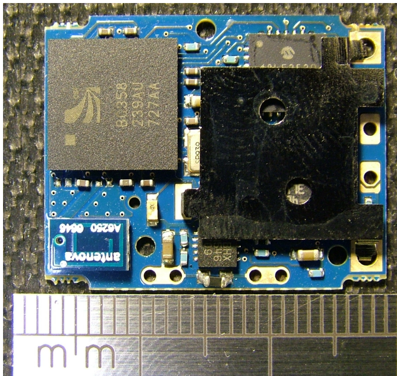
PAM PCB With touch-plate in place
