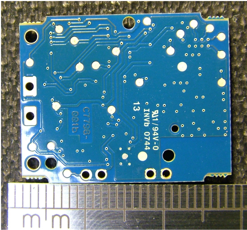
PAM PCB Reverse side
