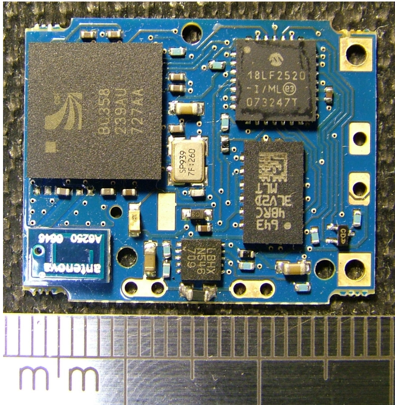
PAM PCB With touch-plate removed
