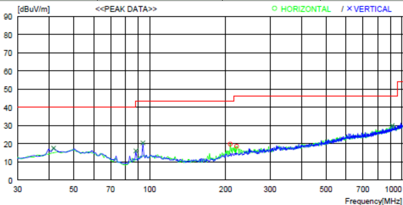
Graphical Test Data – Below 1 GHz – (Bluetooth LE, Low channel)
