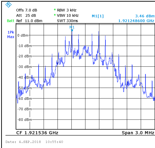
GFSK - Low Channel 1
