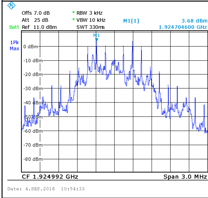
GFSK - Middle Channel 1
