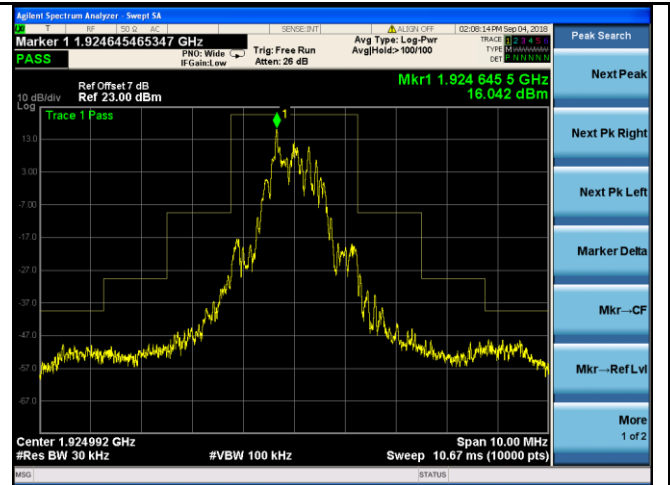
In-band emissions - Middle Channel
