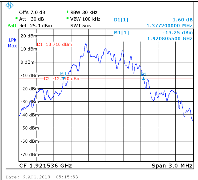
GFSK - Low Channel 26dB
