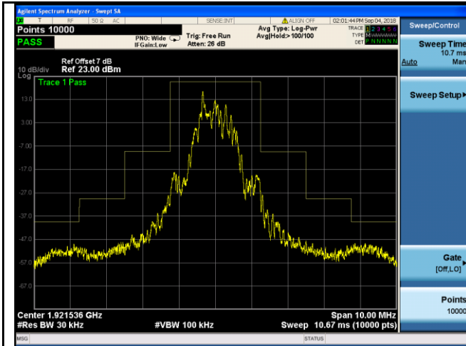
In-band emissions - Low Channel
