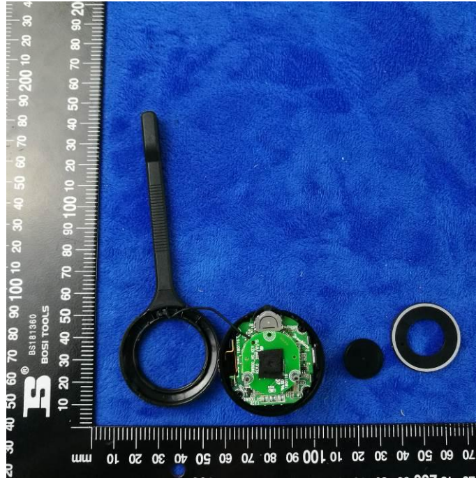
Cover Off - Top View (PP)
