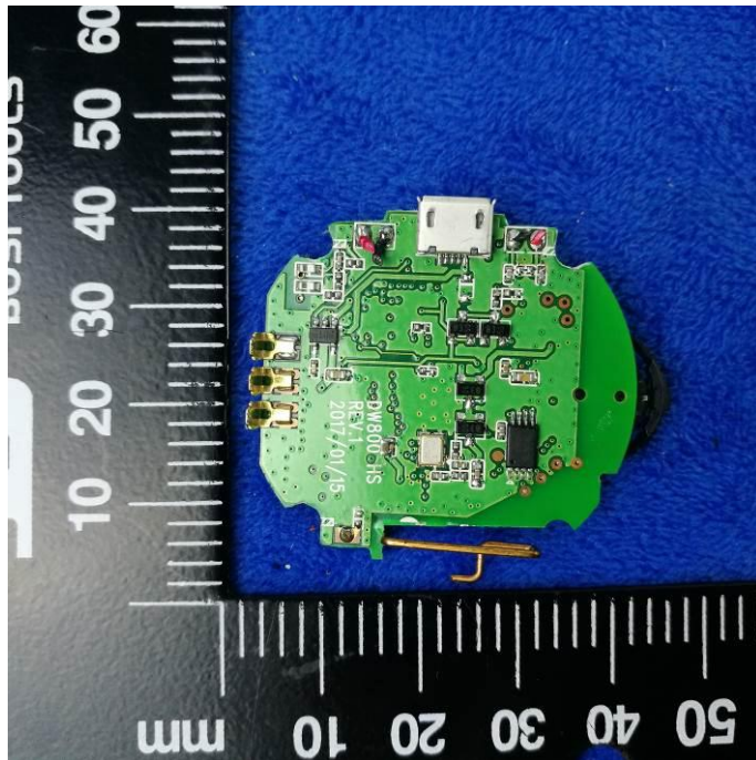
Mainboard - Rear View(PP)
