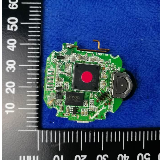
Mainboard - Front View(PP)
