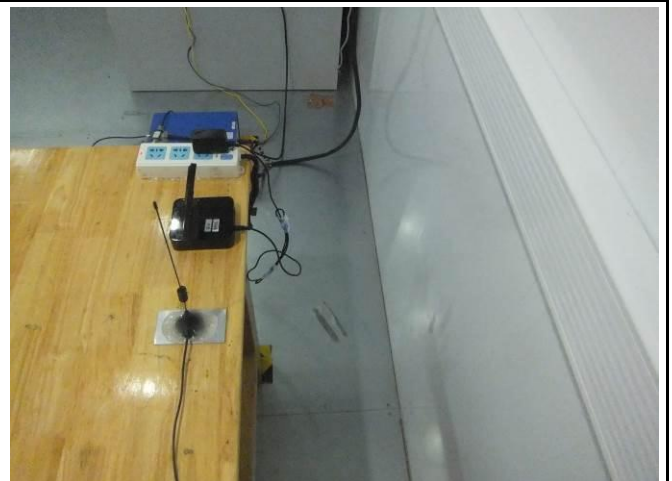
Conducted Emissions Test Setup View 2
