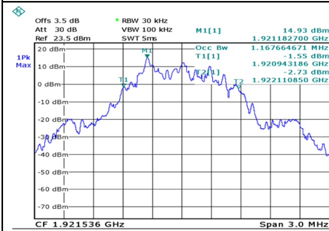
GFSK - Middle Channel 99%
