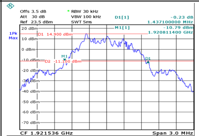
GFSK - Middle Channel 26dB
