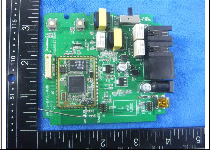
EUT – Mainboard Front View
