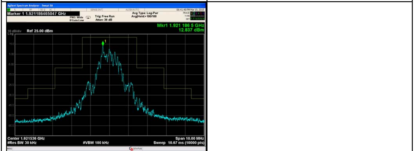
In-band emissions - High Channel
