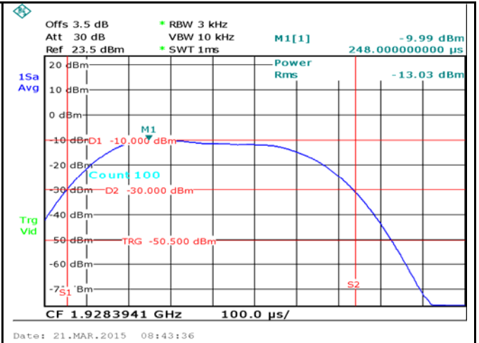
GFSK - Low Channel 2
