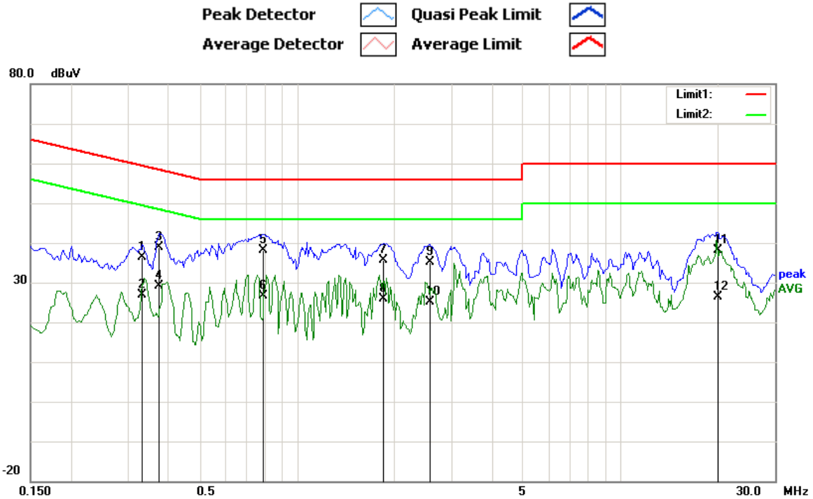
Phase Line Plot at 120Vac, 60Hz
