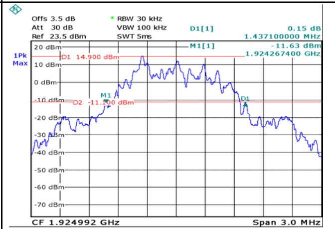
GFSK - Low Channel 26dB
