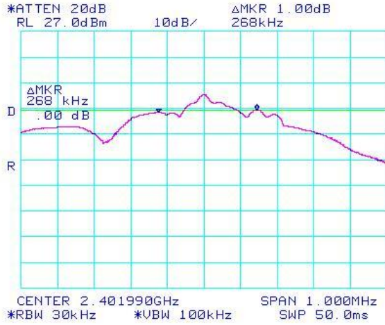
Channel 1 (2 402 MHz)
