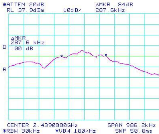
Channel 38 (2 439 MHz)
