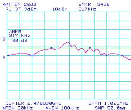
Channel 77 (2 478 MHz)
