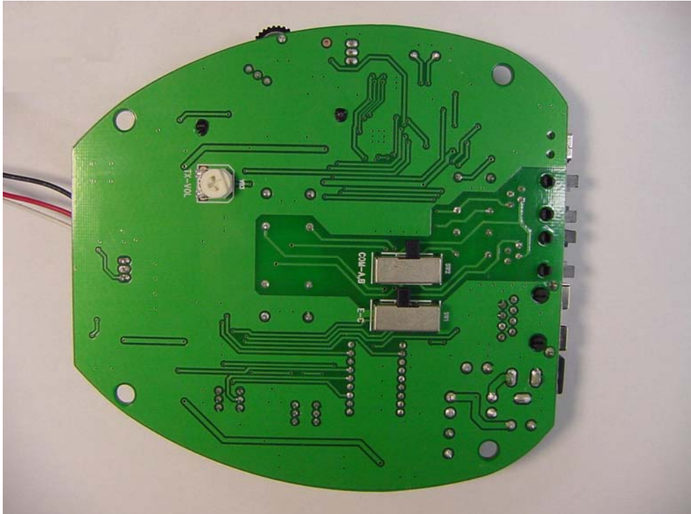
Main board_Port (USB,RJ11, RJ45)
