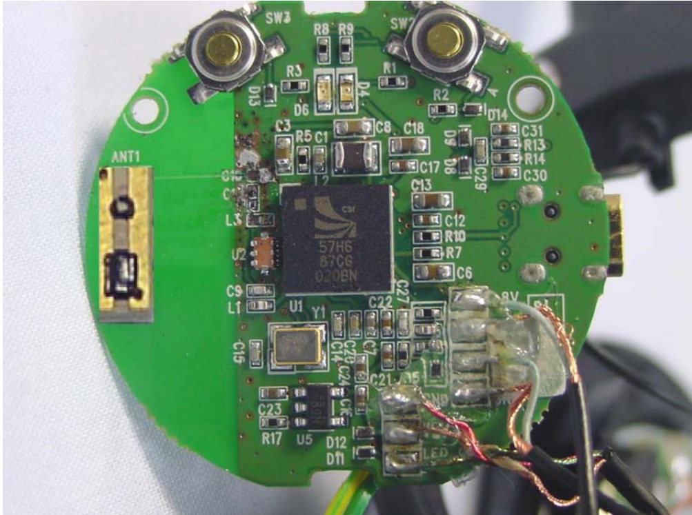
Main board_Rear
