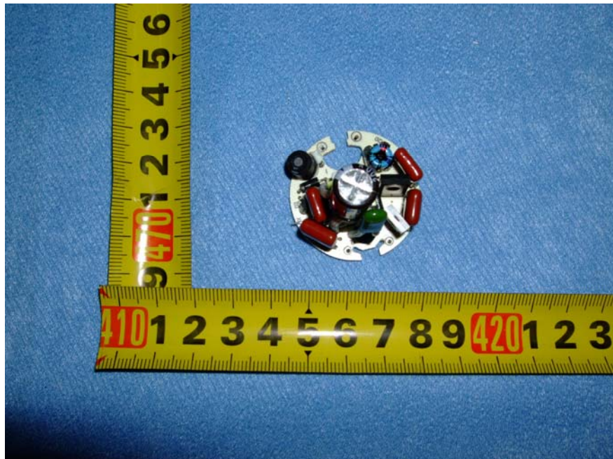
FE224 2012 Main Board - Component Side View
