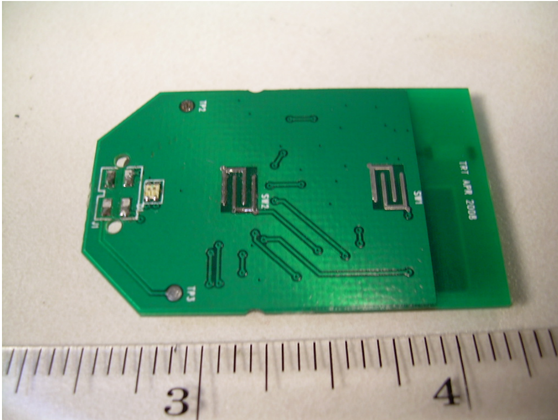
Photograph 7 - View of the Trace Side of the REM-F01 PCB
