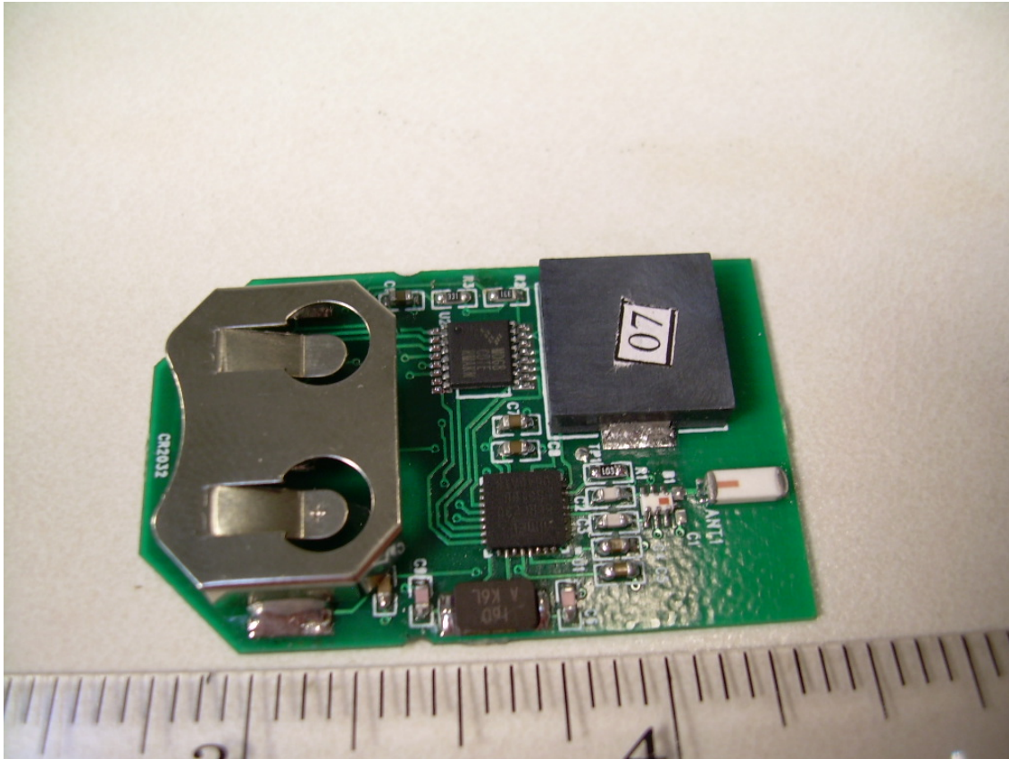
Photograph 6 - View of the Component Side of the REM-F01 PCB
