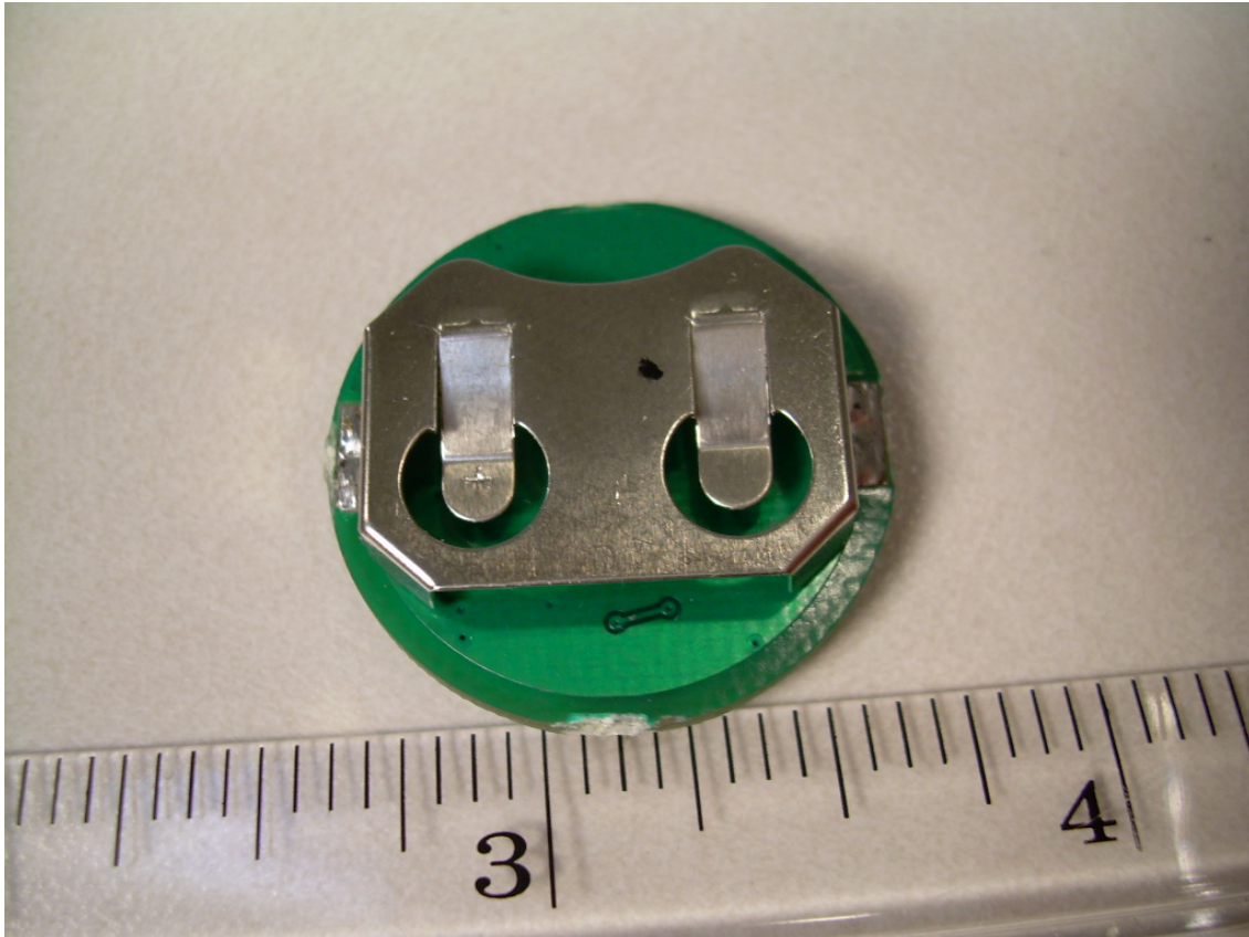
View of the Trace Side of the DSK-A01 PCB
