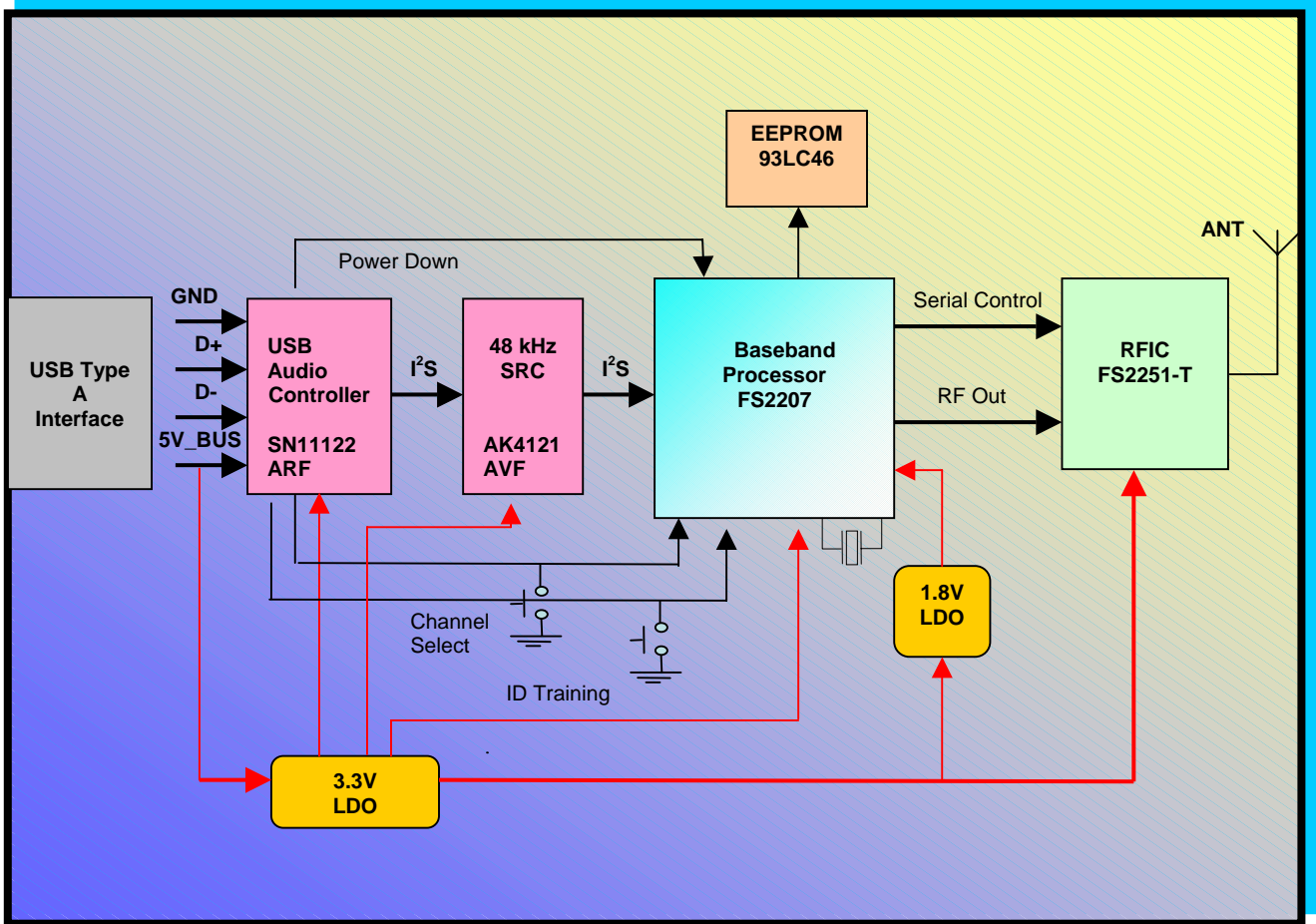
Figure (2) : Wireless USB Audio Transmitter Block Diagram
