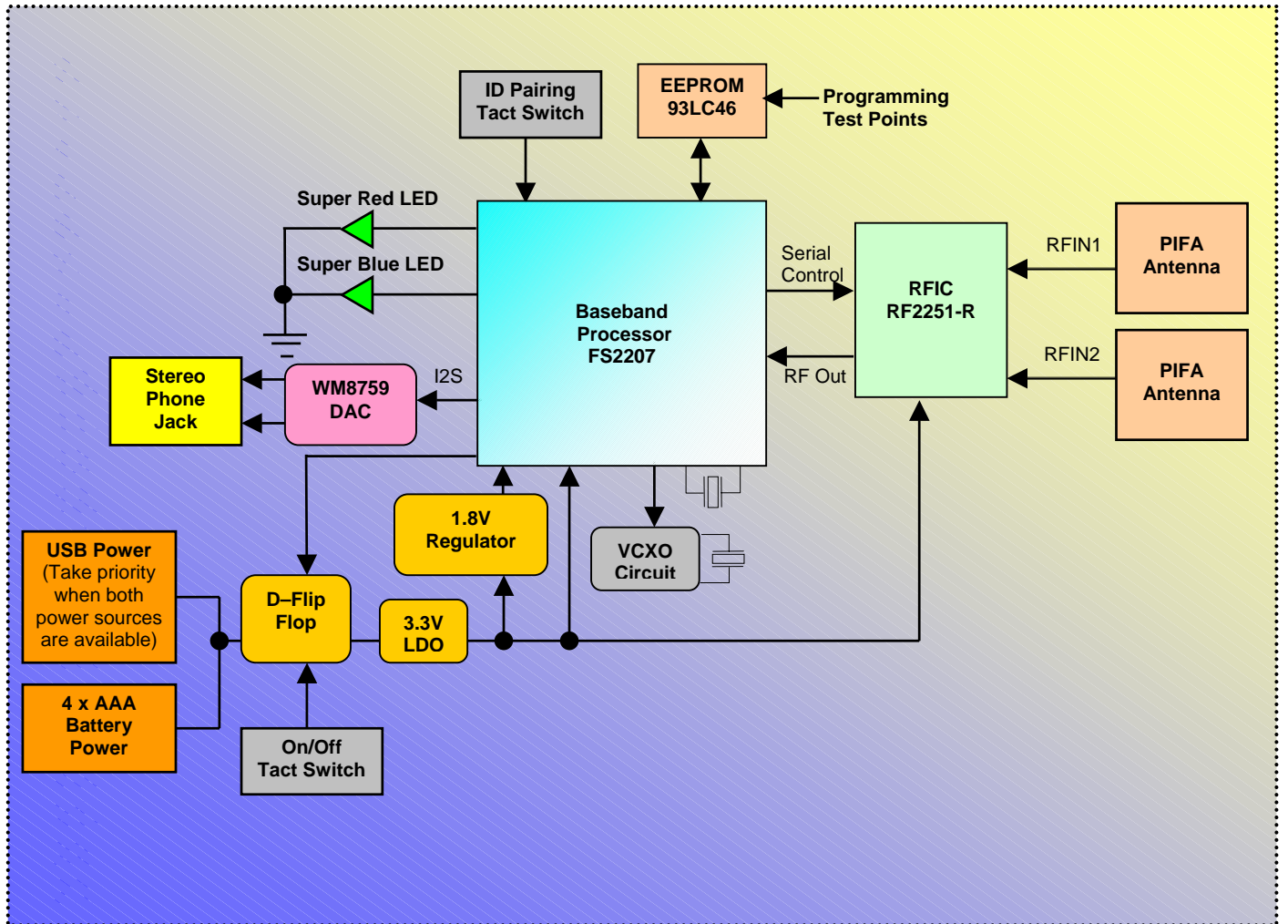
Figure (1) : Receiver Block Diagram
