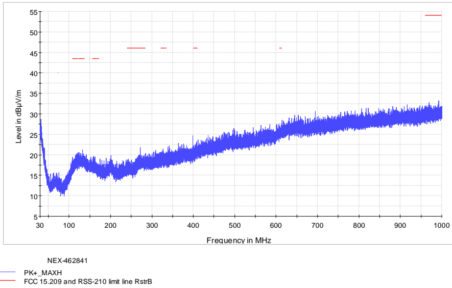
Figure 8.6-12: Radiated spurious emissions 30MHz-1GHz on High Channel
