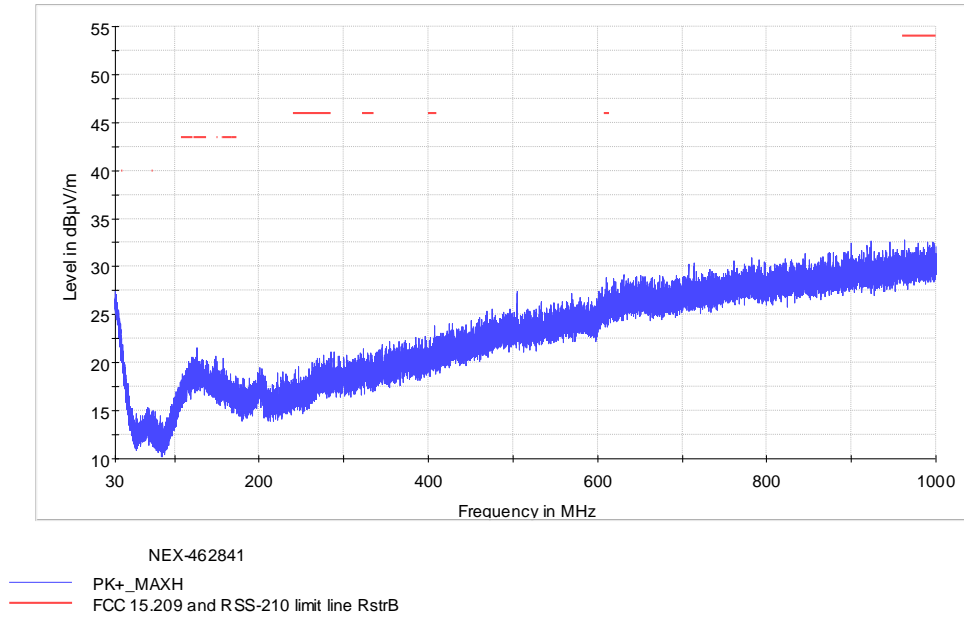
Figure 8.6-10: Radiated spurious emissions 30MHz-1GHz on Low Channel
