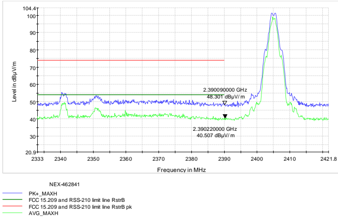
Figure 8.6-6: -Band Edge spurious emissions at 2390 MHz
