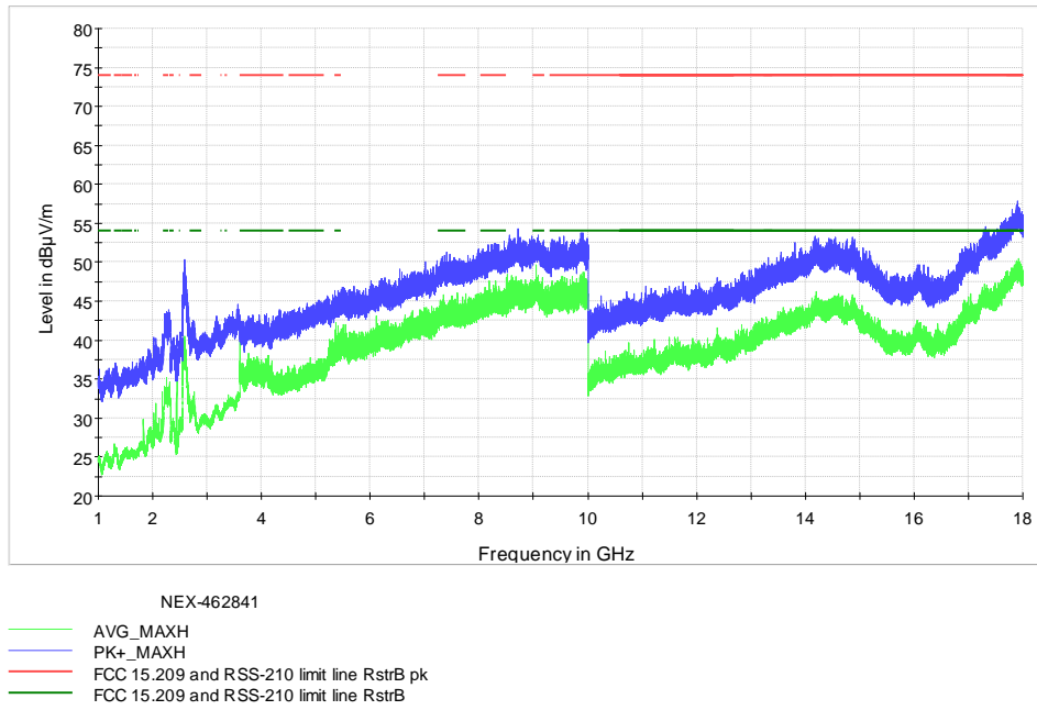
Figure 8.6-14: Radiated spurious emissions 1GHz-18GHz on Mid Channel
