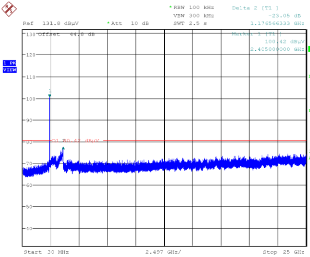
Figure 8.6-1: -20 dBc spurious emissions at 2400 MHz
