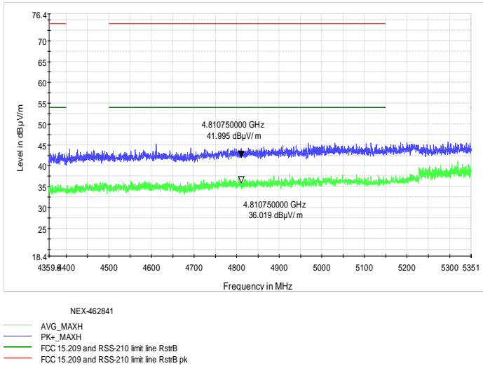
Figure 8.6-8: Radiated spurious emissions at 4810MHz
