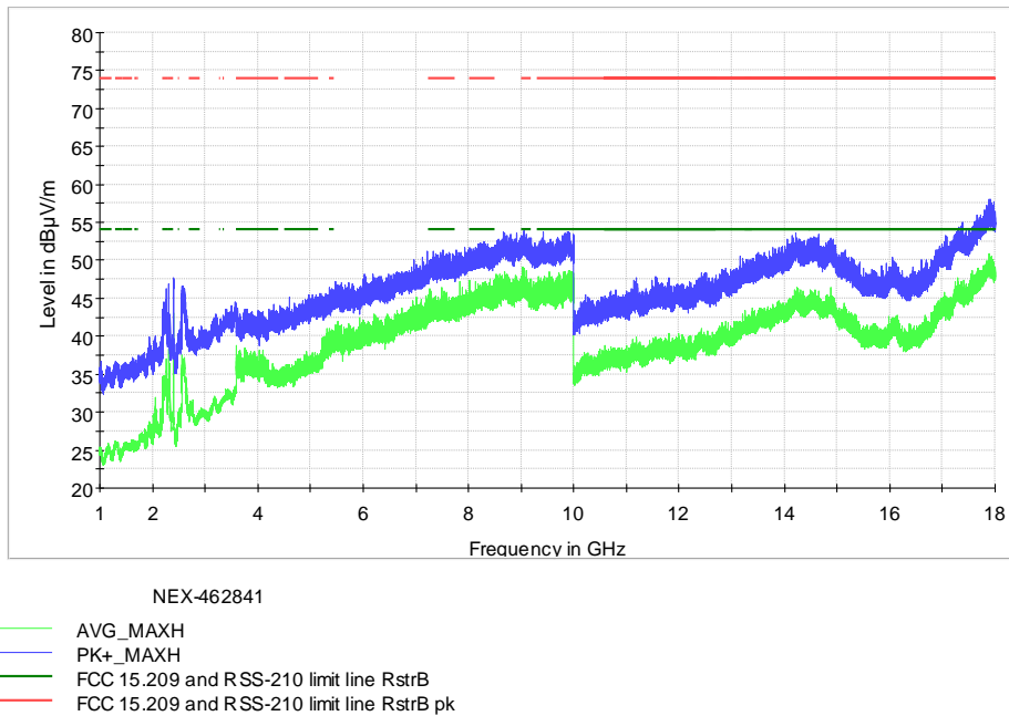
Figure 8.6-13: Radiated spurious emissions 1GHz-18GHz on Low Channel
