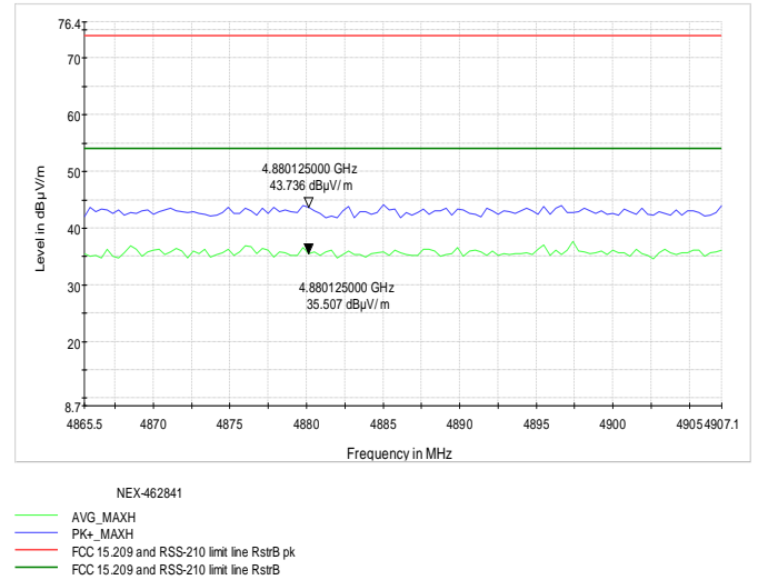
Figure 8.6-9: Radiated spurious emissions at 4880 MHz
