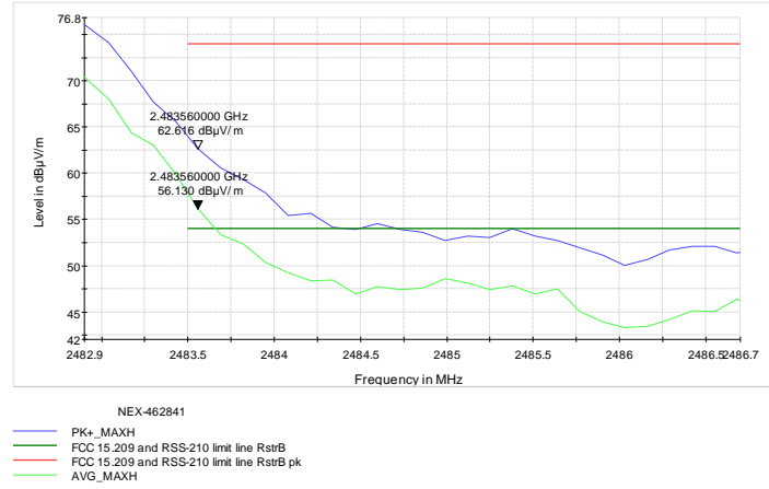
Figure 8.6-7: Band Edge spurious emissions at 2483.5 MHz
