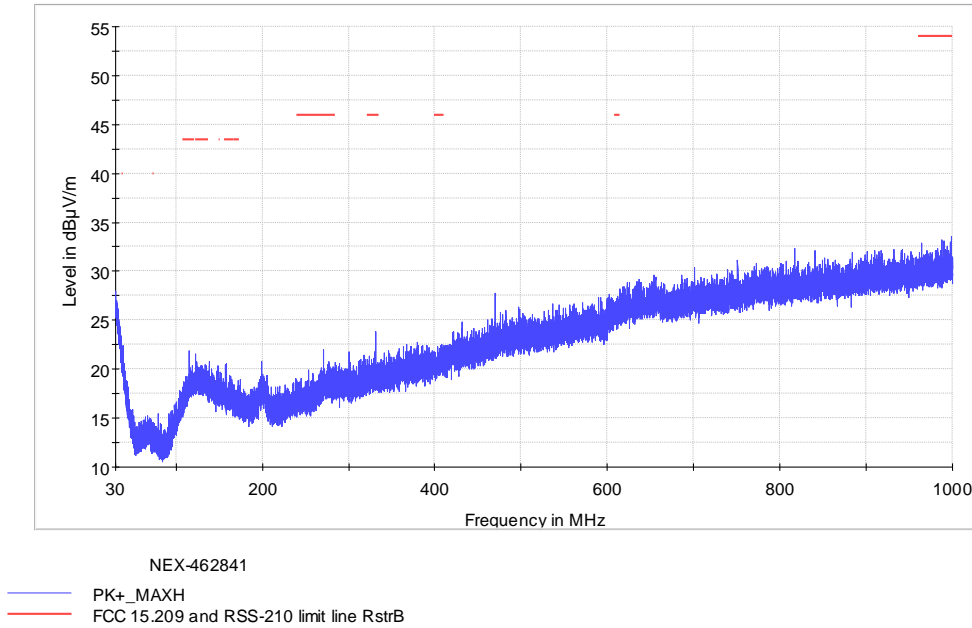
Figure 8.6-11: Radiated spurious emissions 30MHz-1GHz on Mid Channel
