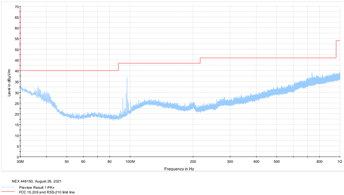
Figure 8.7-11: Radiated spurious emissions 30MHz-1GHz on Mid Channel
