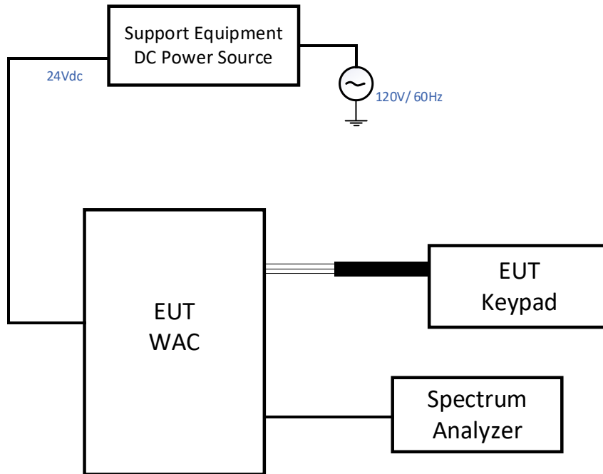
Figure 5.5-2: Antenna port testing block diagram
