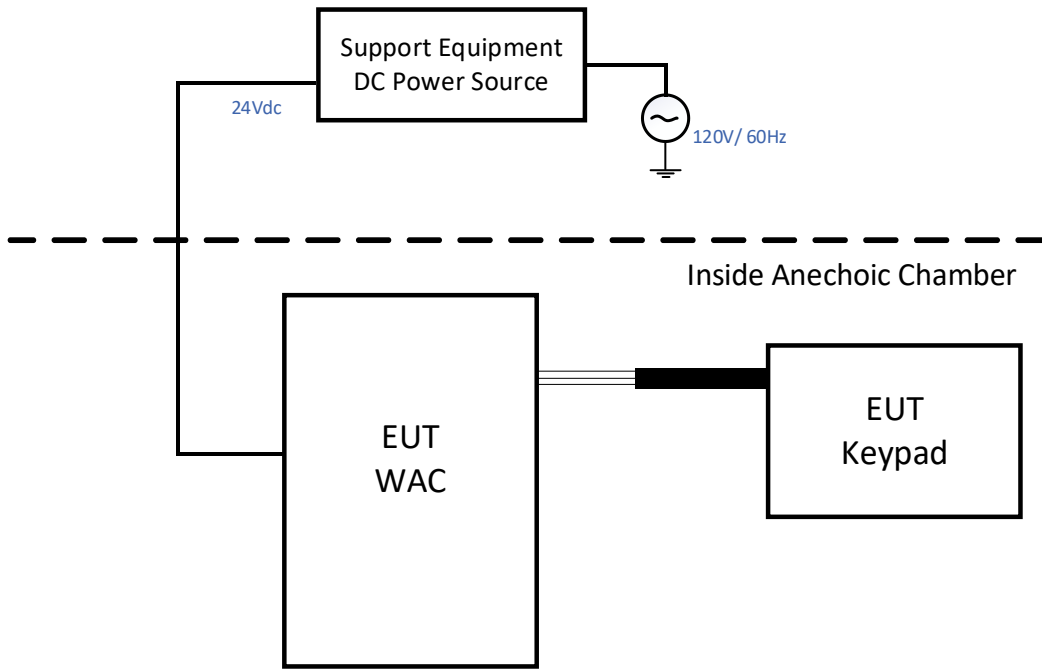
Figure 5.5-1: Testing block diagram
