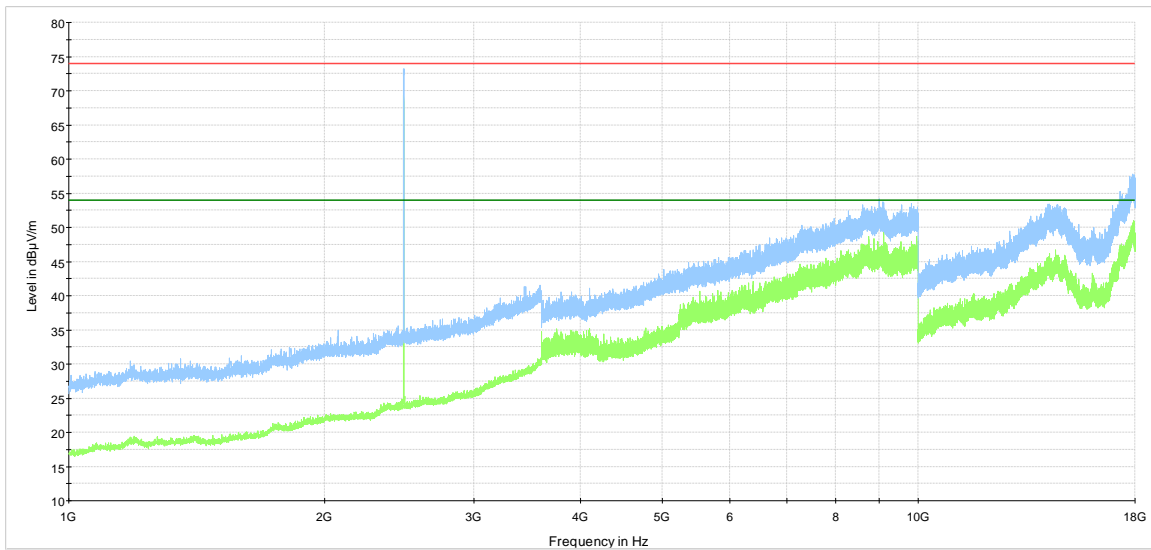
NEX-446150, August 11, 2021 Preview Result 2-AVG Preview Result 1 -PK+ FCC 15.209 and RSS-210 limit line pk FCC 15.209 and RSS-210 limit line
