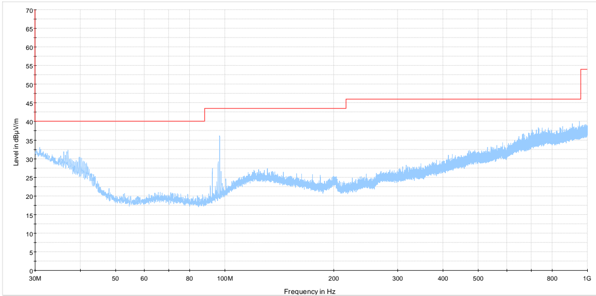
NEX 446150, August 26, 2021 Preview Result 1-PK+ FCC 15.209 and RSS-210 limit line
