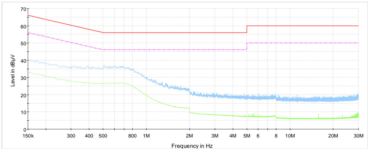
CE 150 KHz to 30 MHz Neutral Preview Result 2-AVG Preview Result 1-PK+ CISPR 32 Limit - Class B, Mains (QP) CISPR 32 Limit - Class B, Mains (Avg)
