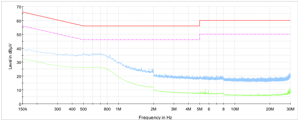
CE 150 kHz to 30 MHz Phase Preview Result 2-AVG Preview Result 1-PK+ CISPR 32 Limit - Class B, Mains (QP) CISPR 32 Limit - Class B, Mains (Avg)
