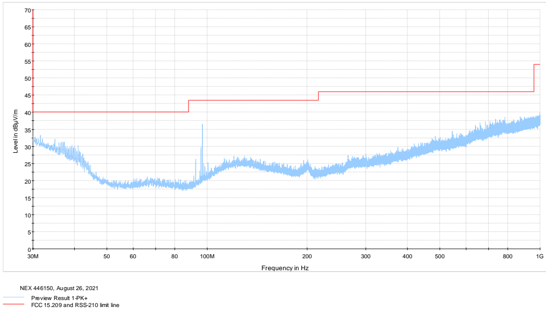
Figure 8.7-10: Radiated spurious emissions 30MHz-1GHz on Low Channel
