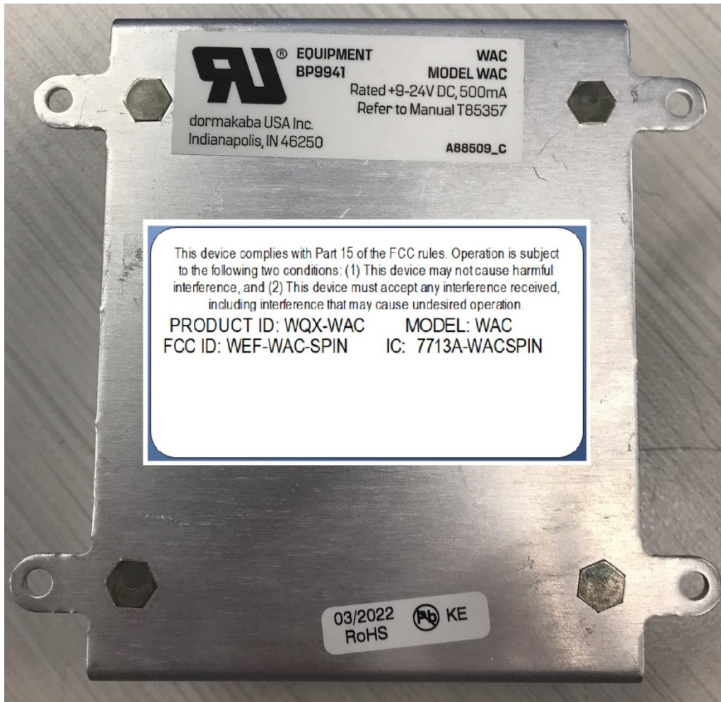
Rear side view
