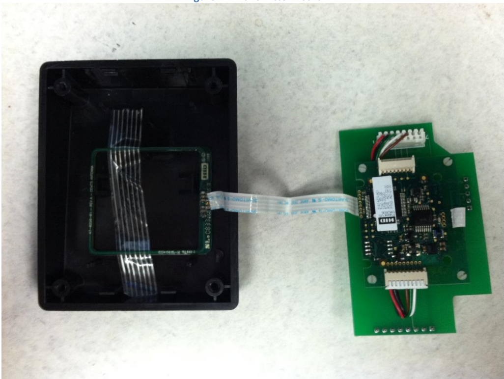
Figure 2 - Transmitter Board and Antenna
