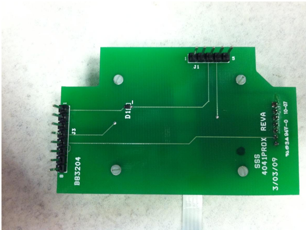
Figure 3 - Back of Transmitter Board
