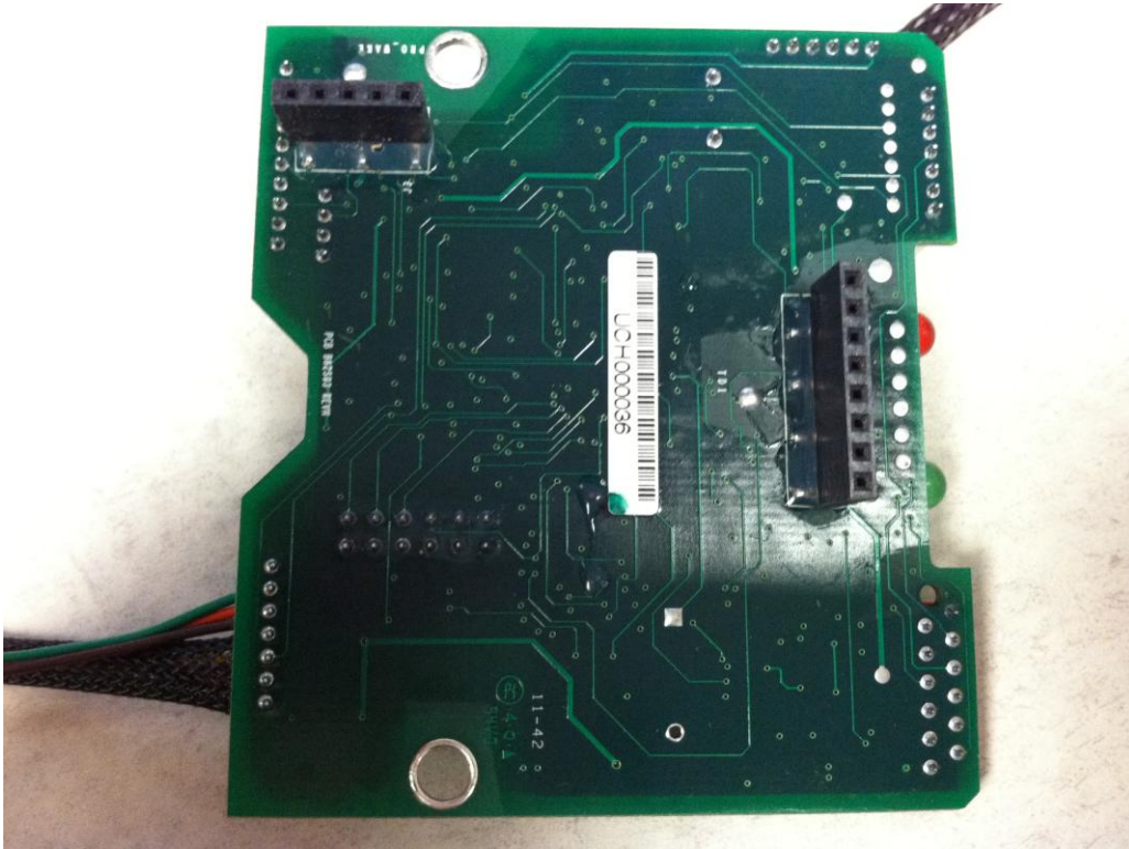
Figure 5 - Back of Main Circuit Board
