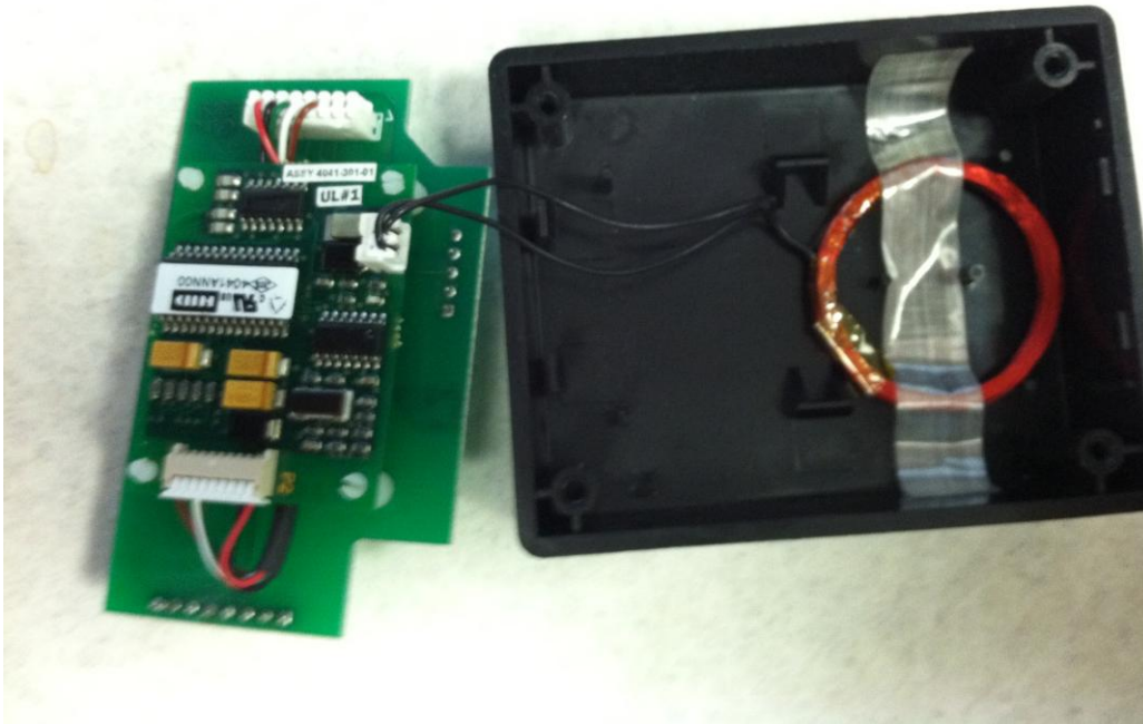
Figure 1 - Transmitter Board and Antenna
