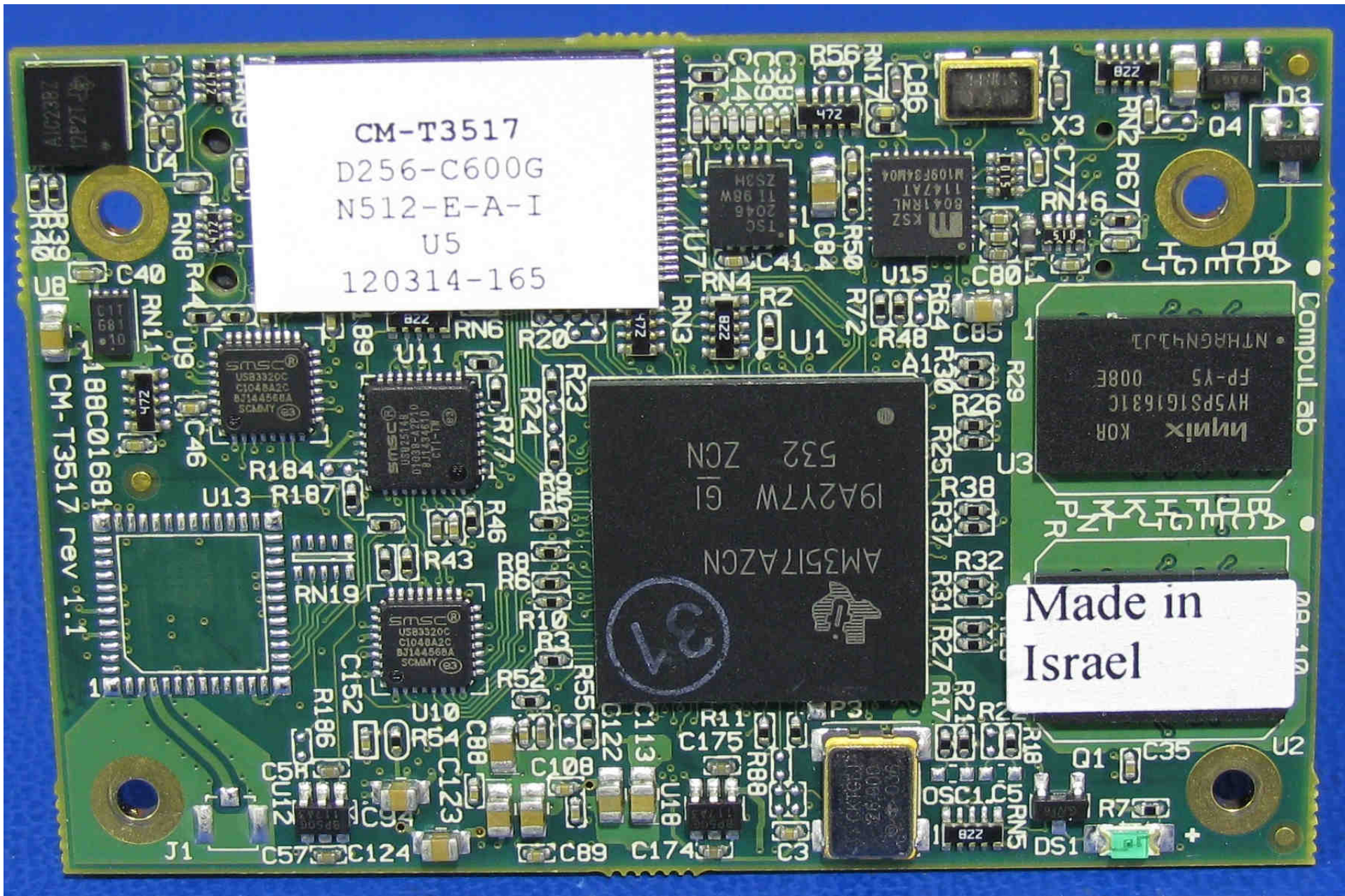
Daughter Card, Top Side
