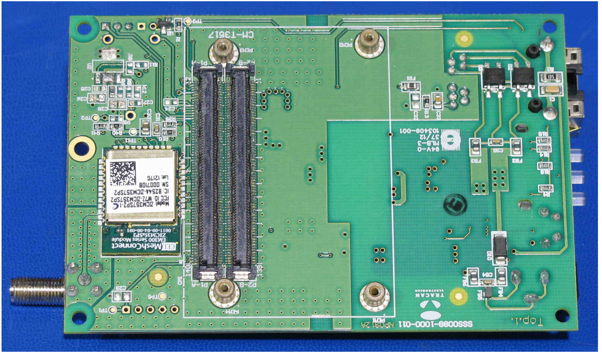
Mother Card, Bottom Side
