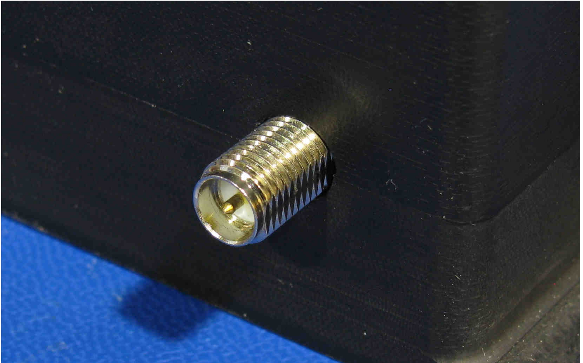
Reverse Polarity SMA Connector
