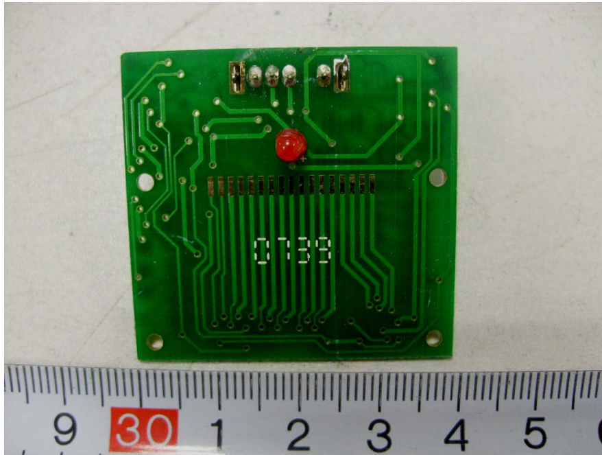
EUT - RF Board Front View
