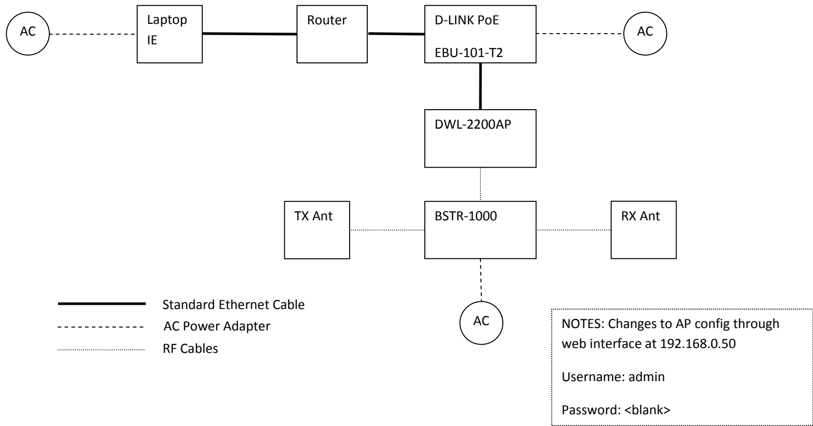
Figure 1 SPK-1000 Test Setup
