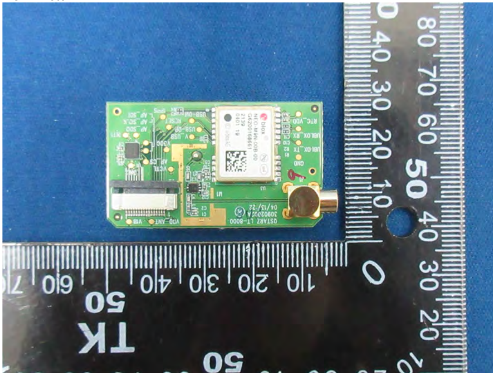
(18) EUT Photo – GNSS Internal Antenna
