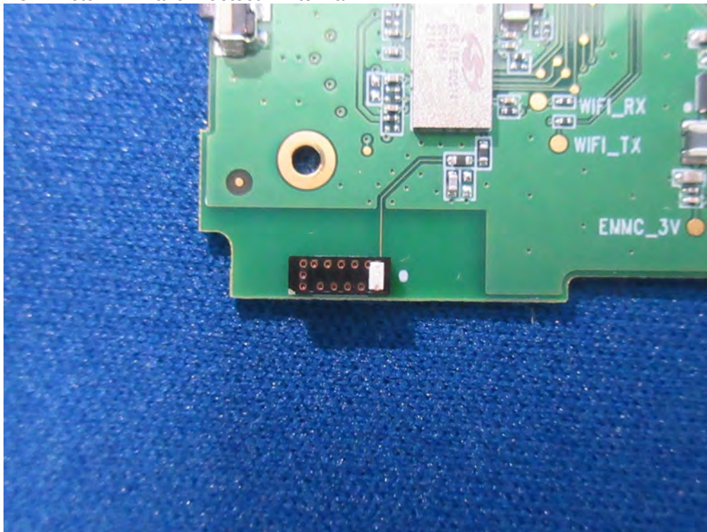
(10) EUT Photo - WiFi and Bluetooth Antenna
