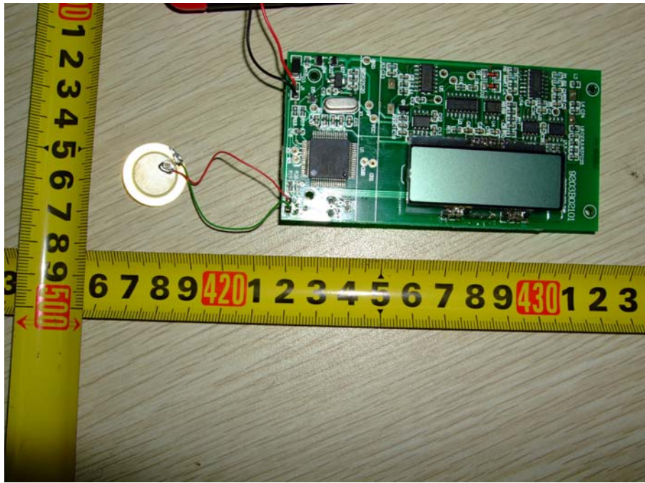
9203 Main Board Component View
