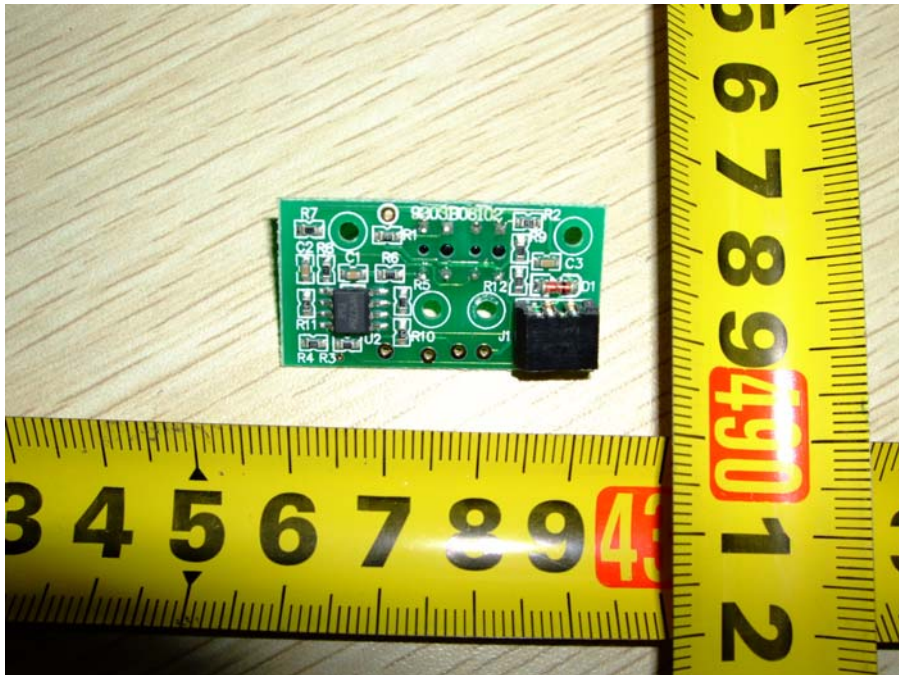
9203 Motor Board #1 Component View
