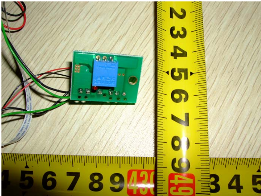
9203 Motor Board #2 Soldered View
