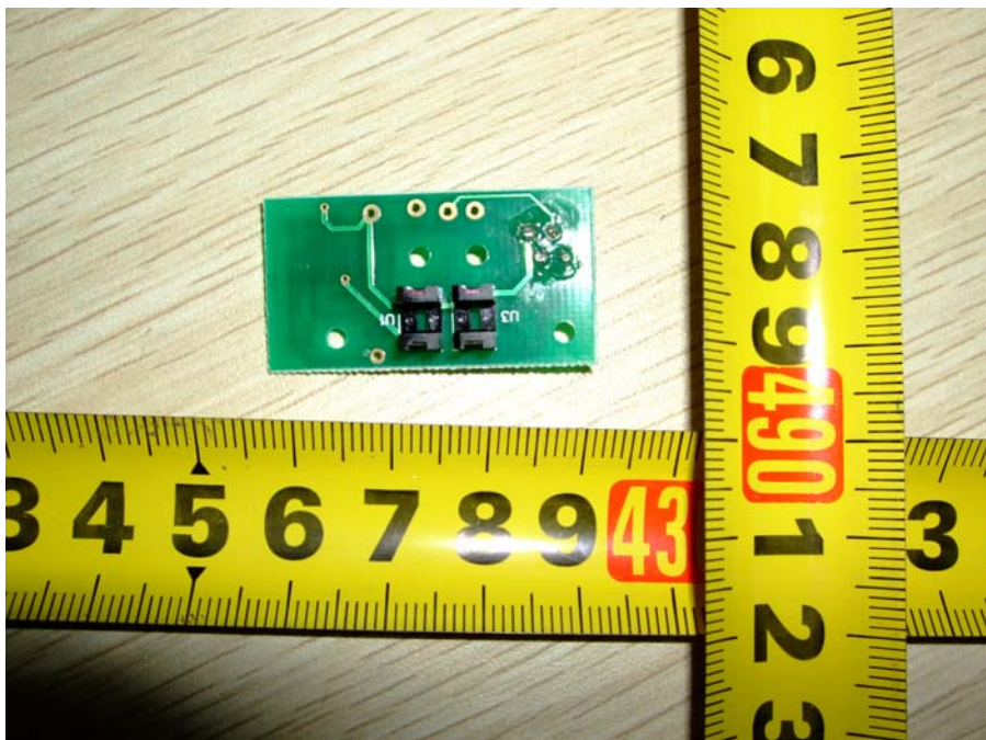
9203 Motor Board #1 Soldered View
