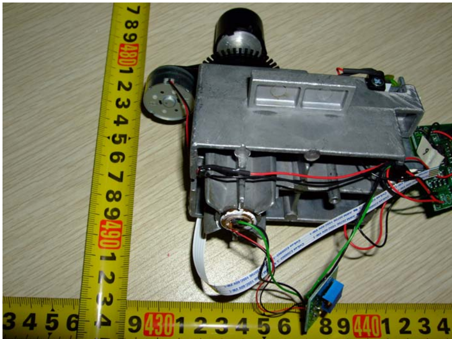
9203 Motor Back View
