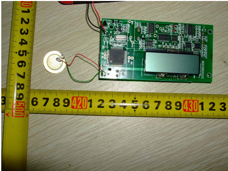
9203 Detector Board Component View
