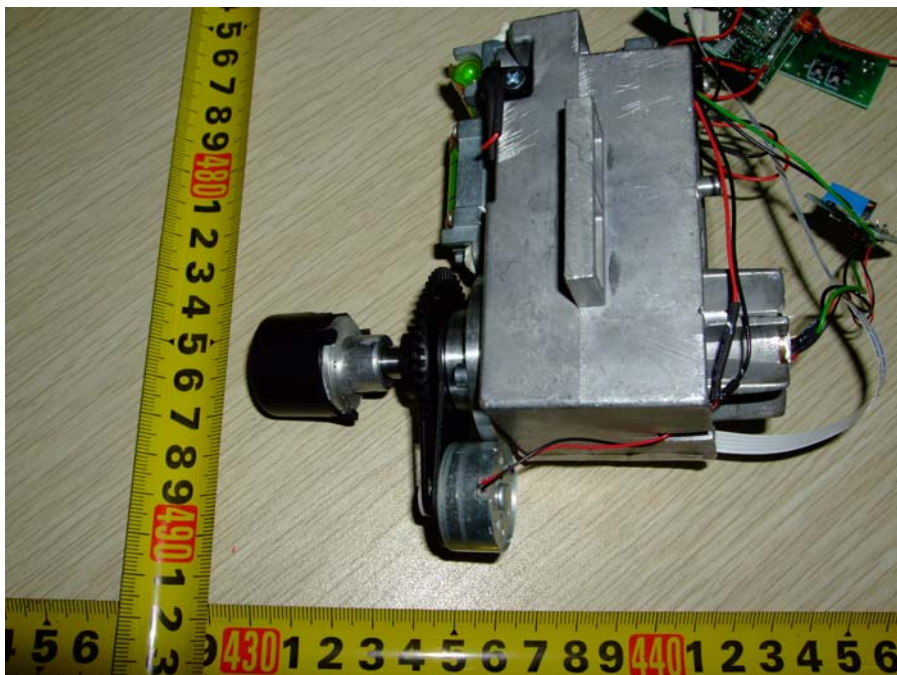
9203 Motor Right View
