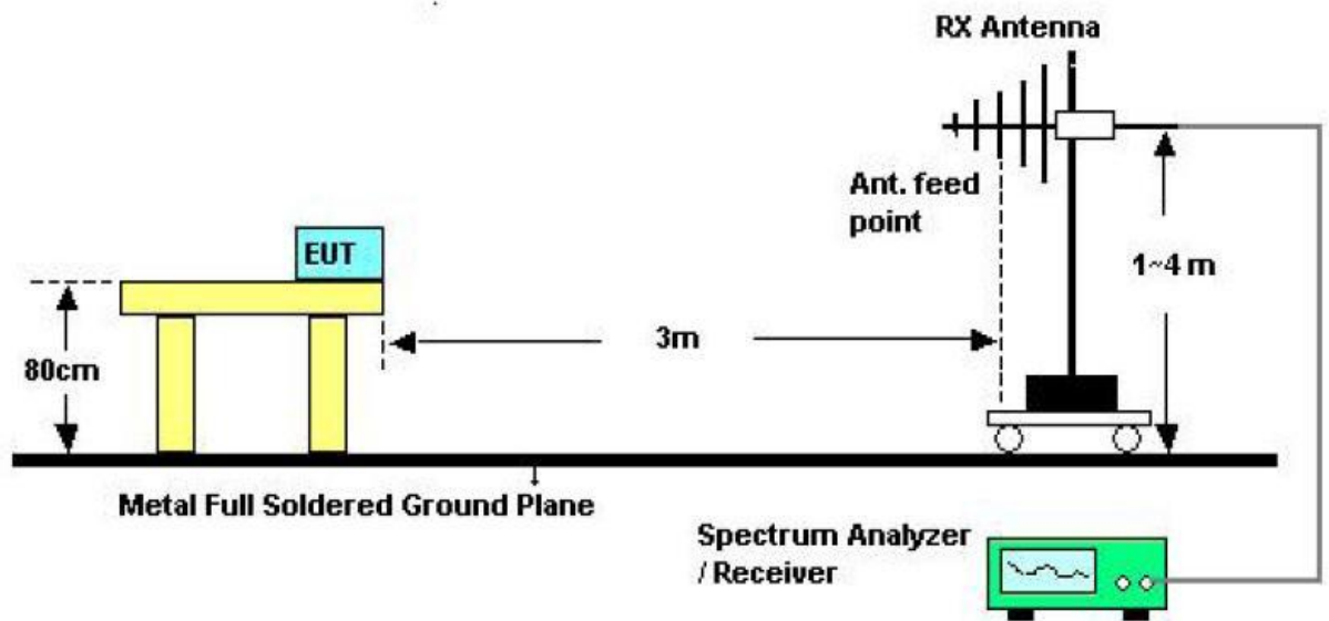
Test Setup for Emission above 30MHz
