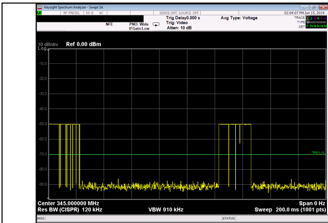
Figure 1 Pulse Train >100ms
