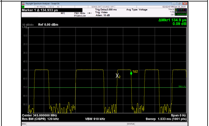
Figure 4 Small Pulse Duration
