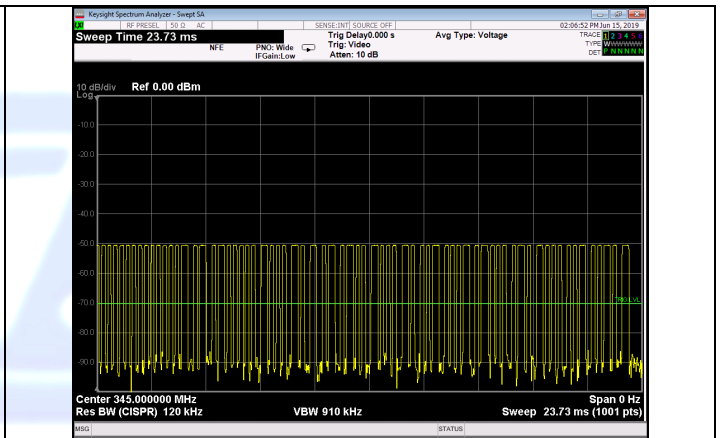
Figure 2 Sum by Pulse Type
