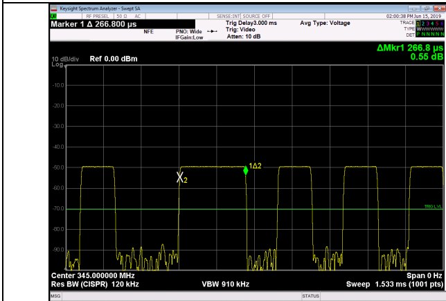
Figure 3 Large Pulse Duration
