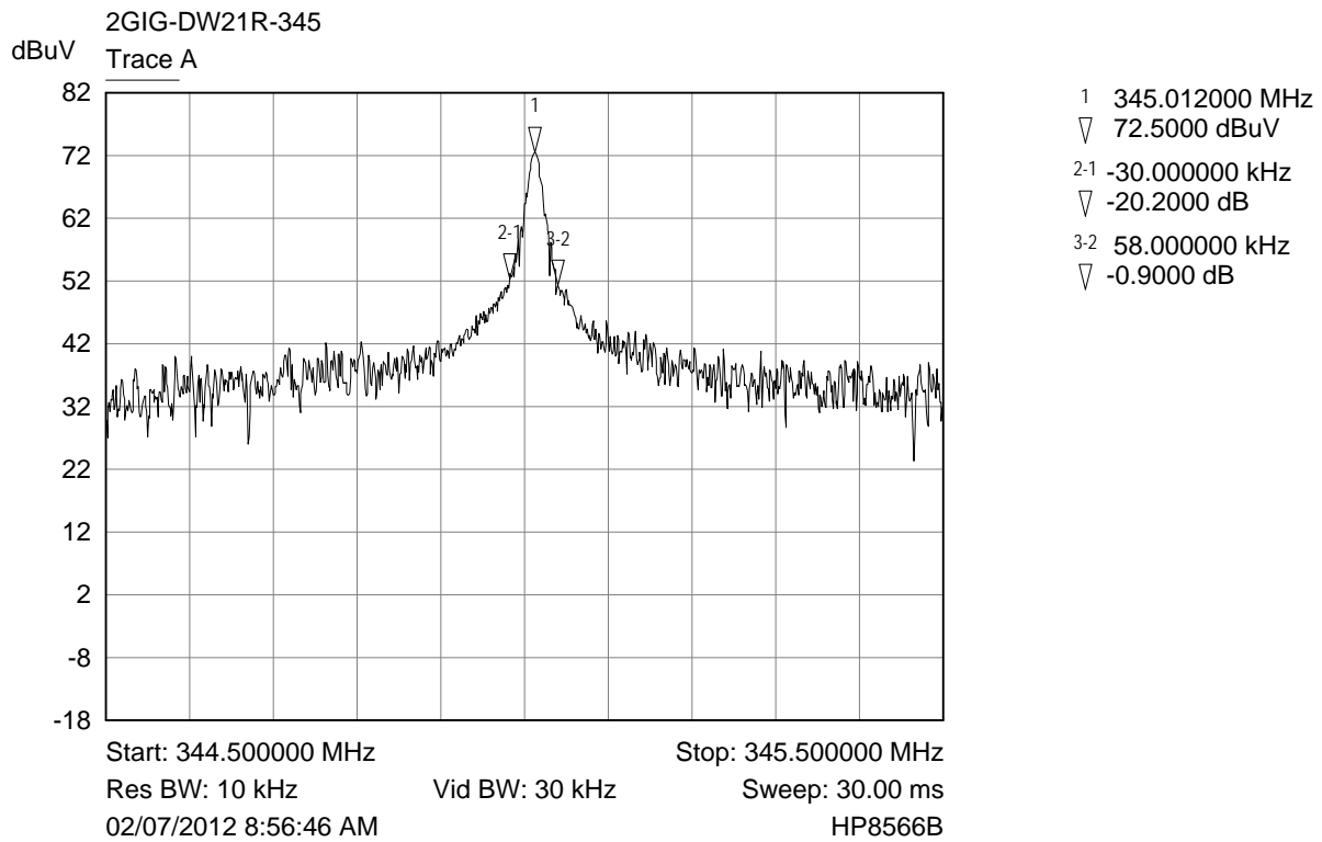
Bandwidth Plot
