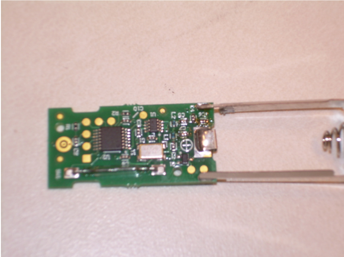
Photograph 4 – View of the Component Side of the PCB
