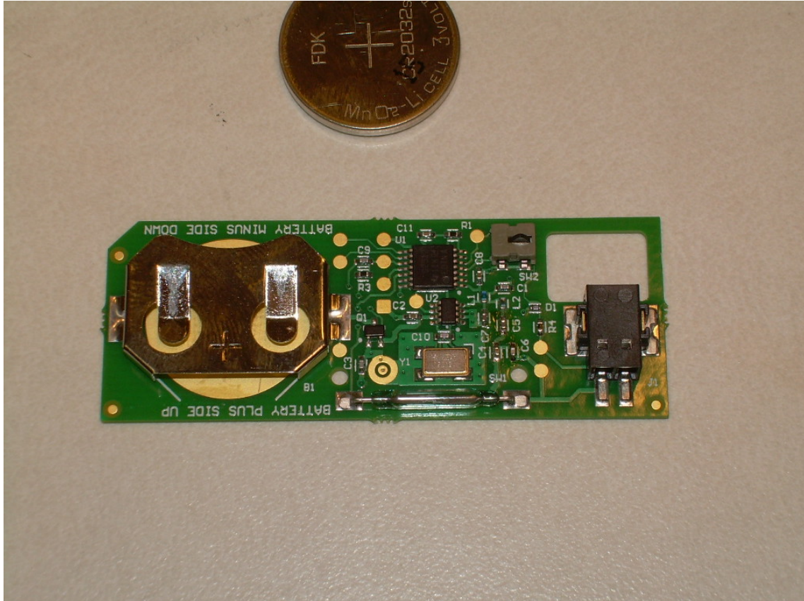
Photograph 5 – View of the Component Side of the PCB
