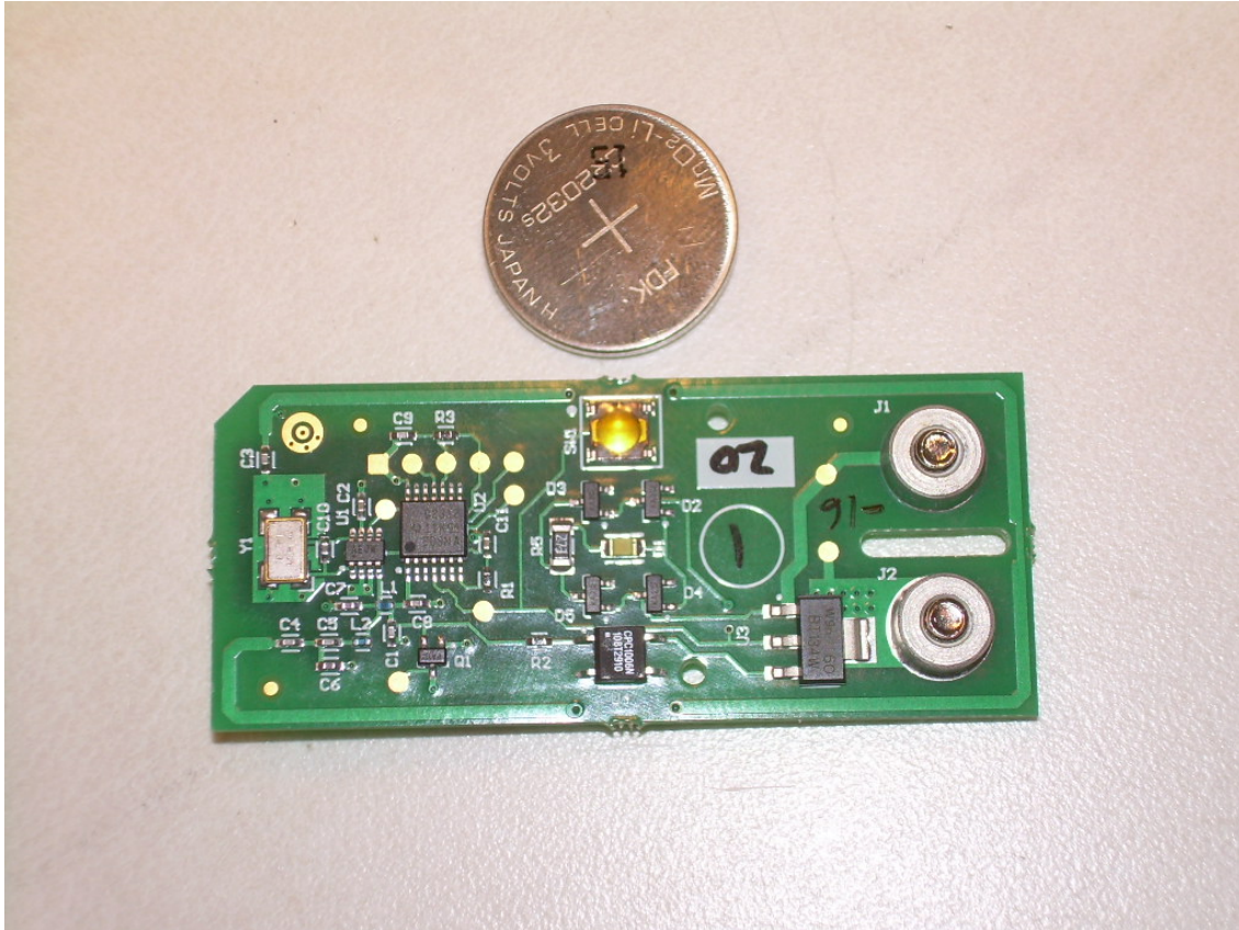
Photograph 6 – View of the Component Side EUT PCB
