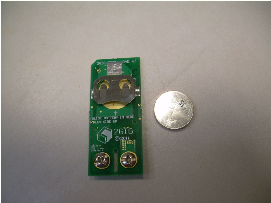
Photograph 7 – View of the Trace Side of the EUT PCB
