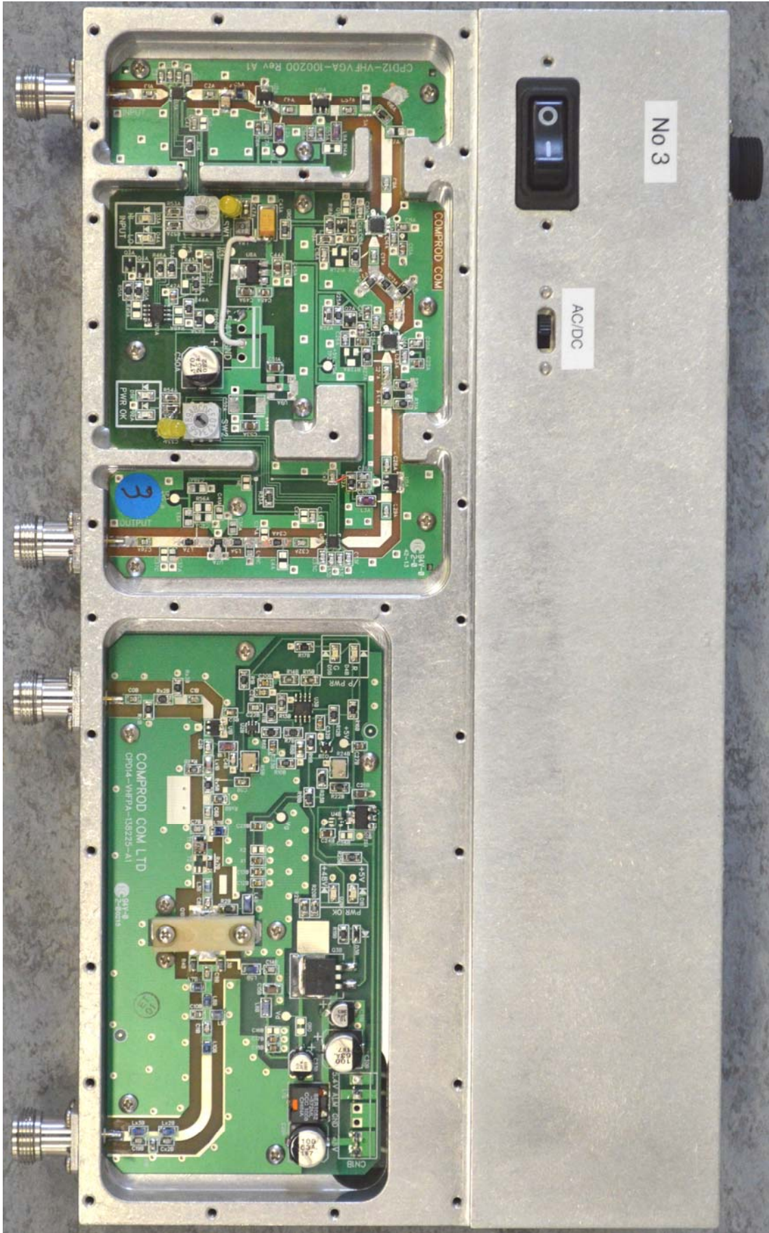
Comprod Communications Ltd VHF Uni-Directional Amplifier, Model UDA138225 IC: 7755A-UDA138225
