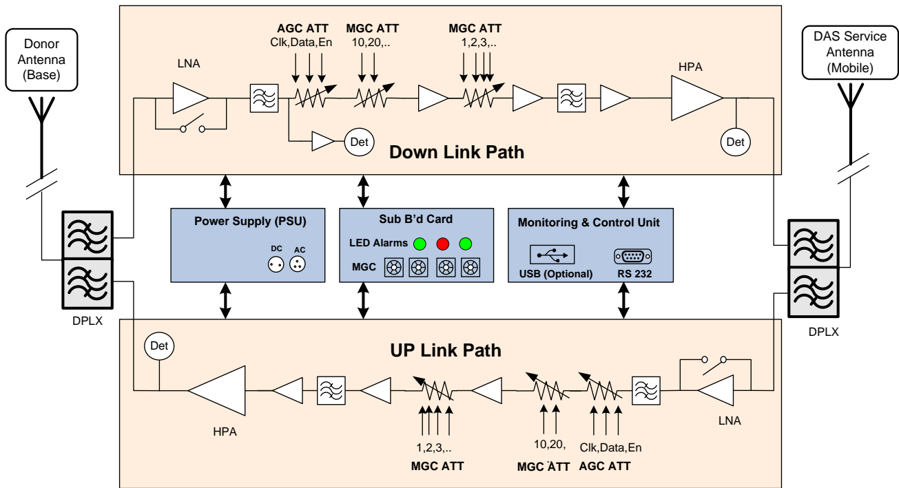
Figure 1: Block diagram of the 800 MHz bidirectional amplifier
