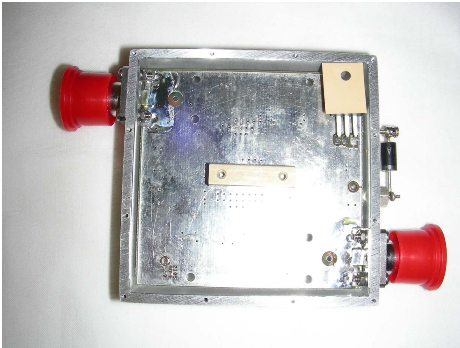
Comprod Communications VHF Signal Booster Class B, Model 08US1008 FCC ID: WDM-08US1008, IC: 7755A-08US1008
