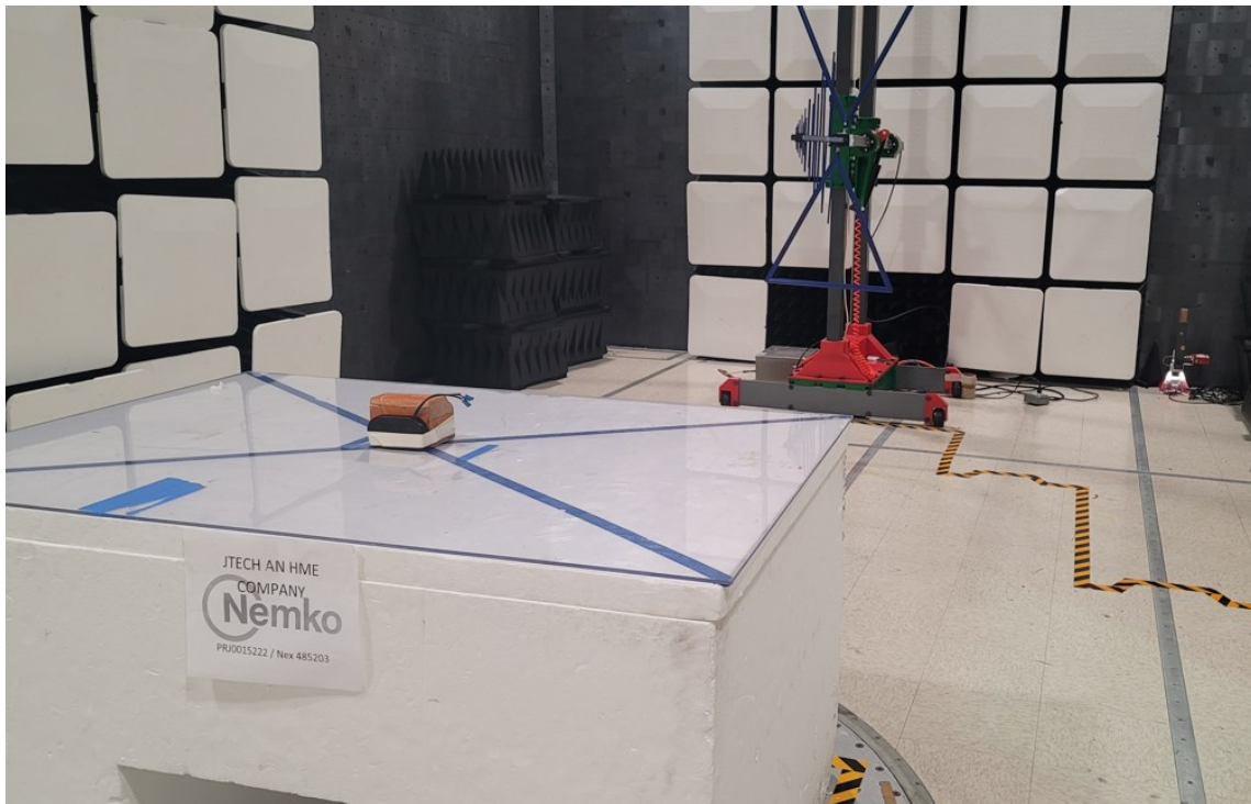
Figure 3 - Radiated emissions below 1 GHz (0.03 – 1 GHz), rear view.
