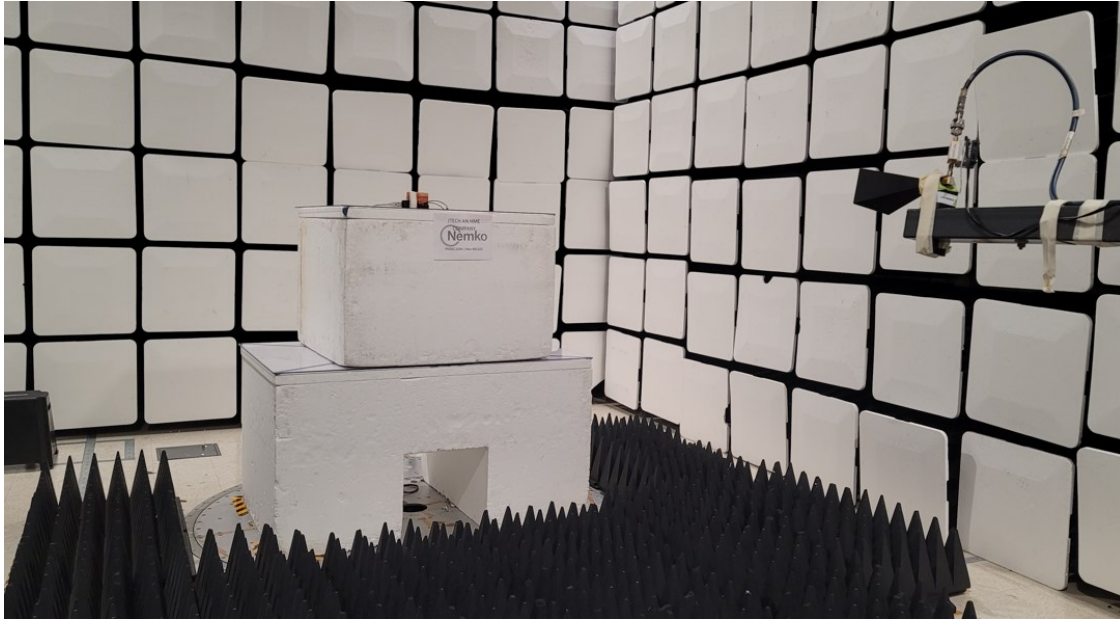
Figure 6 - Radiated emissions above 1 GHz (18 – 26 GHz), front view.
