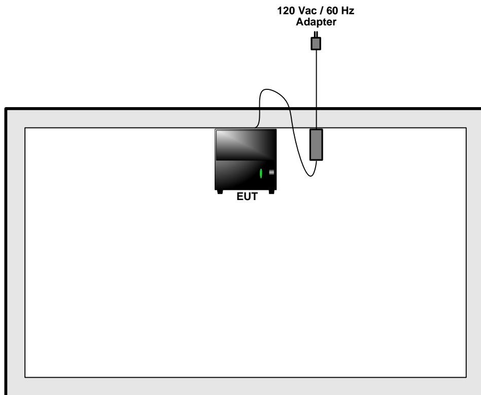
Test Setup Diagram - Radiated Above 30MHz Test
